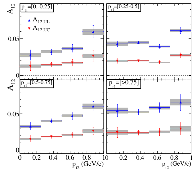
Figure 24.1.13. Preliminary BABAR results (Garzia, 2013) on azimuthal asymmetries measured from fits to the R^U/R^L ( A_{12,UL} ), and R^U/R^C ( A_{12,UC} ) ratios, as functions of the transverse momentum p_{t2} for four bins of p_{t1} , from top left to bottom right. Statistical and systematic errors are shown as errors bars and shaded bands respectively.
