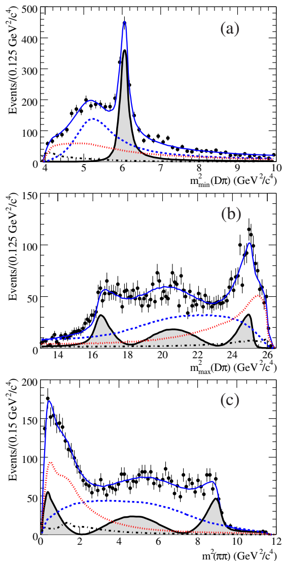
Figure 19.3.4. From (Aubert, 2009g). Result of the Dalitz plot fit to the B^- \rightarrow D^+\pi^-\pi^- signal candidates: projections on (a) m_{\min}^2(D\pi) , (b) m_{\max}^2(D\pi) and (c) m^2(\pi\pi) . The points with error bars are data, the solid curves represent the nominal fit. The shaded areas show the D_2^{*0} contribution, the dashed curves show the D_0^{*0} signal, the dash-dotted curves show the D_v^* and B_v^* signals, and the dotted curves show the background.
