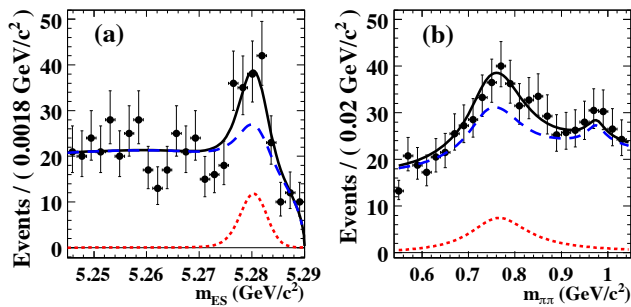
Figure 17.7.7. Projections of the multidimensional fit of the BABAR \rho^0 \rho^0 analysis (Aubert, 2008r) onto the (a) m_{ES} , and (b) di-pion invariant mass (combining the m(\pi\pi)_1 and m(\pi\pi)_2 distributions), after a requirement on the signal-to-background probability ratio calculated using all discriminating variables excluding the one plotted, which enhances the fraction of signal events in the sample. This selection has 40% (60%) efficiency for signal for the m_{ES} ( m_{\pi\pi} ) projection. The data points are overlaid by the full p.d.f. projection (solid black line). Also shown are the B^0 \rightarrow \rho^0 \rho^0 p.d.f. component (dotted line) and the sum of all other p.d.f.s (dashed line).
