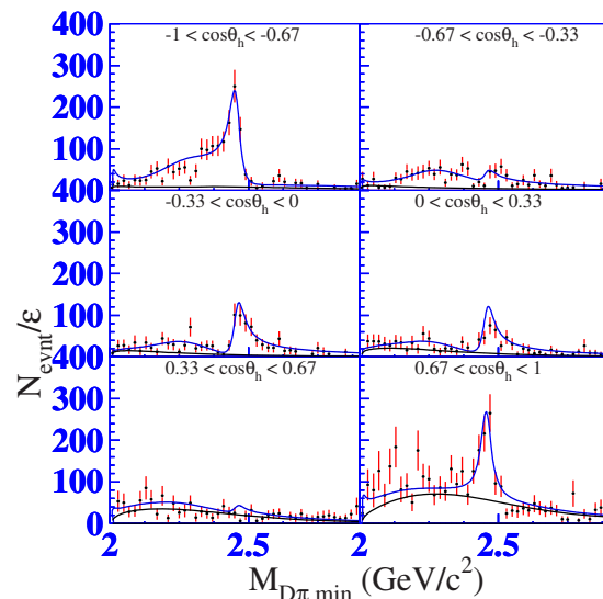
Figure 19.3.5. From (Abe, 2004f). Efficiency-corrected M(D^+\pi^-)_{\min} distribution in B^- \rightarrow D^+\pi^-\pi^- for different helicity angle ranges. Curves correspond to the fit to the total distribution (upper blue) and background (lower black) component.
