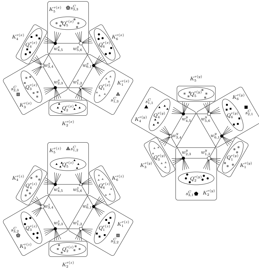
Figure 2: Parts of clusters for variables x, y and z with \phi'(x) = 1, \phi'(y) = 0, \phi'(z) = 1 , and a clause C = (\neg x \vee \neg y \vee z) with \text{var}(C, 1) = x, \text{var}(C, 2) = y, \text{var}(C, 3) = z and \eta(C) = 2 (note that both y and z satisfy C in the assignment \phi' , but y was chosen as a representative).
