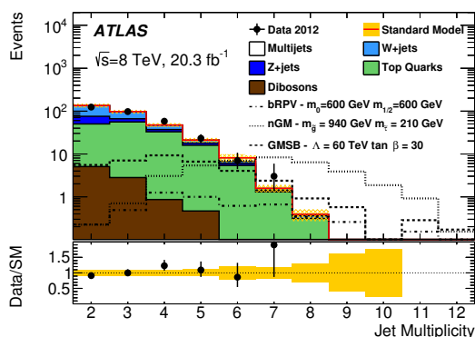
(c) 2\tau N_{\text{jet}} distribution.
