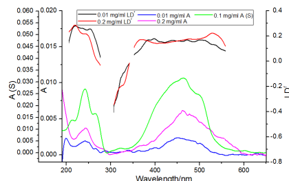
Figure 3 (a) LD spectra of 9-methyl-2,3,7-trihydroxy-6-fluorone on PE OX deposited from 0.01 and 0.2 mg/mL solution and stretched by a factor of \times 2.4 . \parallel and \perp indicate transition polarization with respect to the xanthene long axis in Figure 2. (b) Absorbance and LD f spectra of the LD spectra in Figure 3(a) overlaid with solution absorbance spectrum (denoted S).
