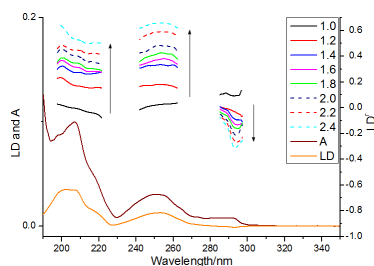
Figure 2. Spectra of xanthene on PE OX dropped from a 0.2 mg/mL solution onto an unstretched film and then stretched (stretch factor as indicated in inset). \parallel and \perp indicate transition polarization with respect to the xanthene long axis in Figure 2. (a) LD, (b) LD f calculated as indicated in Methods overlaid with absorbance and LD spectra of \times 2.4 stretched PE OX .
