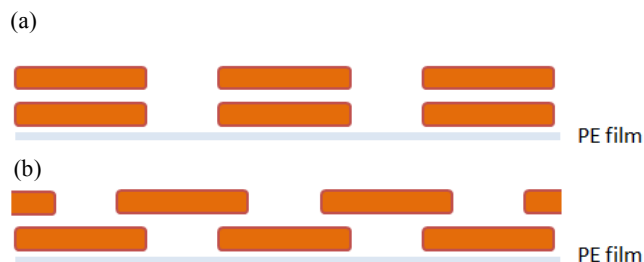
Figure 8 (a) H-aggregate geometry which is consistent with the data for MeOH 3 -fluorone and pyronin Y at high concentrations. (b) Offset stacked geometry which is consistent with the data for pyronin B, fluorescein, and rhodamine 6G at high concentrations.
