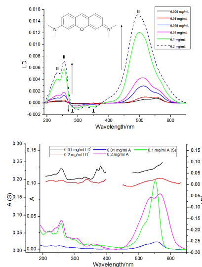
Figure 5 (a) LD spectra of pyronin B on PEOX deposited from solutions of concentrations indicated in the Figure. // and \perp indicate transition polarization with respect to the xanthene long axis in Figure 2. (b) Absorbance and LD spectra of samples with concentrations 0.01 and 0.2 mg/ml overlaid with solution absorbance spectrum (S) and the dimer/monomer difference spectrum.
