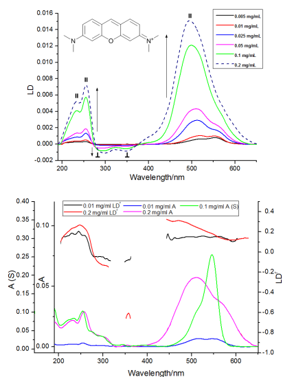
Figure 4 (a) LD spectra of pyronin Y on PEOX deposited from solutions of concentrations indicated in the Figure. // and \perp indicate transition polarization with respect to the xanthene long axis in Figure 2. (b) Absorbance and LD spectra of samples with concentrations 0.01 and 0.2 mg/ml overlaid with solution absorbance spectrum (S) and the dimer/monomer difference spectrum.
