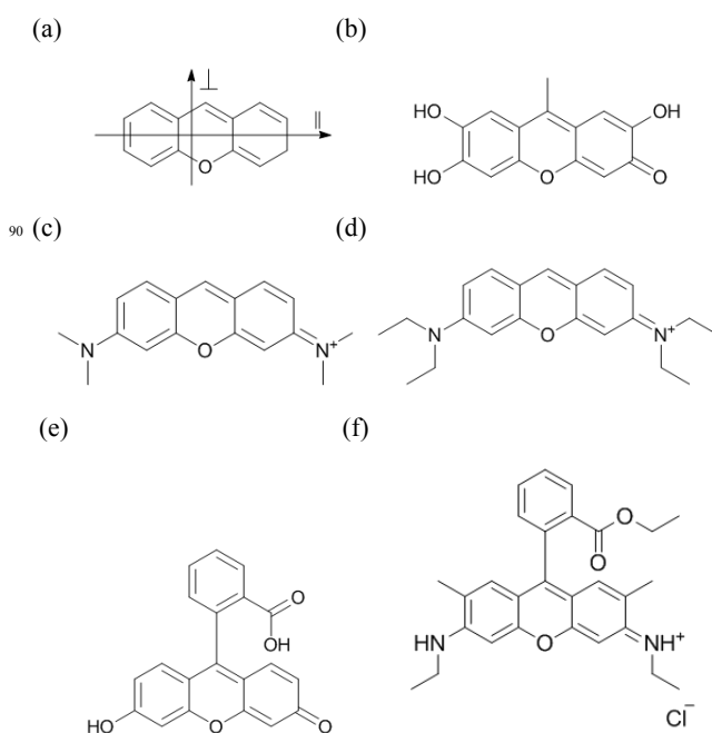
Figure 1. (a) Xanthene with z and y axes indicated by // and ⊥ respectively, (b) 9-methyl-2,3,7-trihydroxy-6-fluorone, (c) pyronin Y, (d) pyronin B, (e) fluorescein, and (f) rhodamine 6G.
