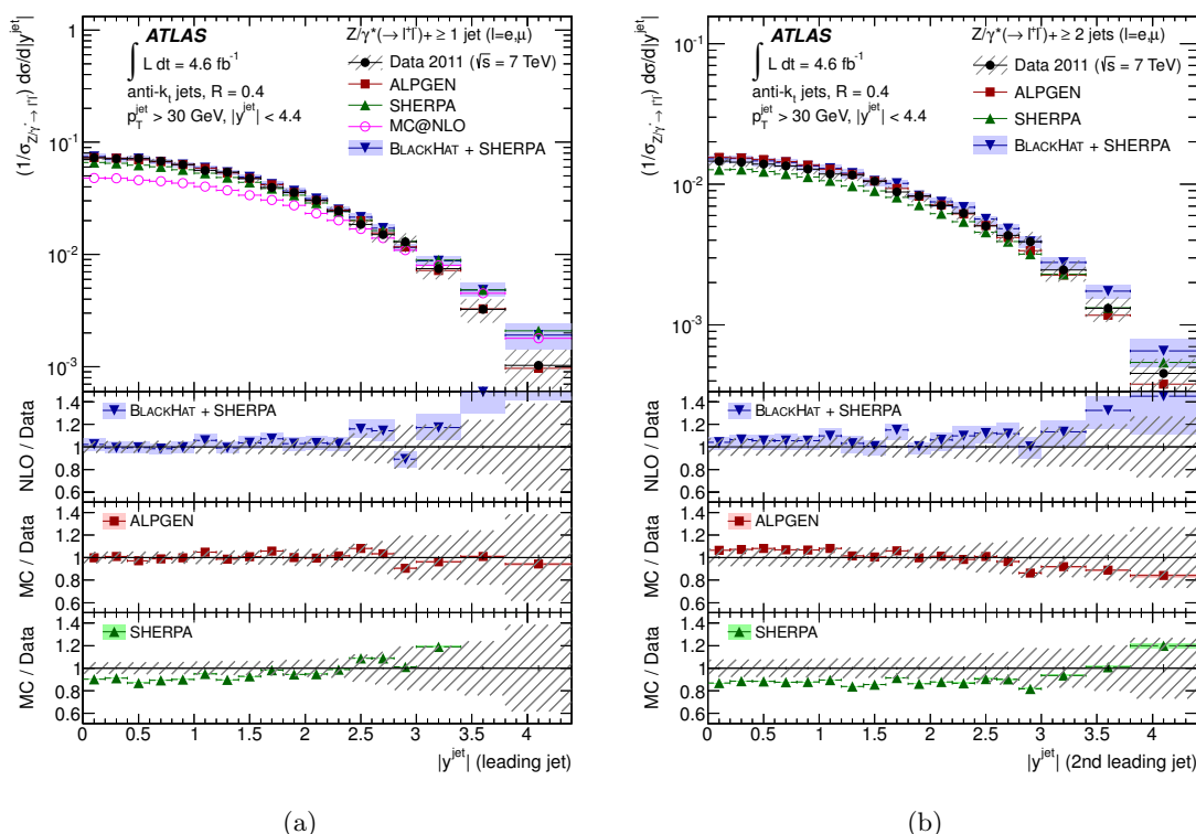
Figure 9. (a) Measured cross section for Z (\rightarrow \ell\ell) + \text{jets} as a function of the absolute value of the rapidity, |y^{\text{jet}}| , of the leading jet for events with at least one jet with p_T^{\text{jet}} > 30 GeV and |y^{\text{jet}}| < 4.4 in the final state and (b) as a function of |y^{\text{jet}}| of the second leading jet for events with at least two jets. The cross sections are normalized to the inclusive Z (\rightarrow \ell\ell) cross section. The other details are as in figure 2.
