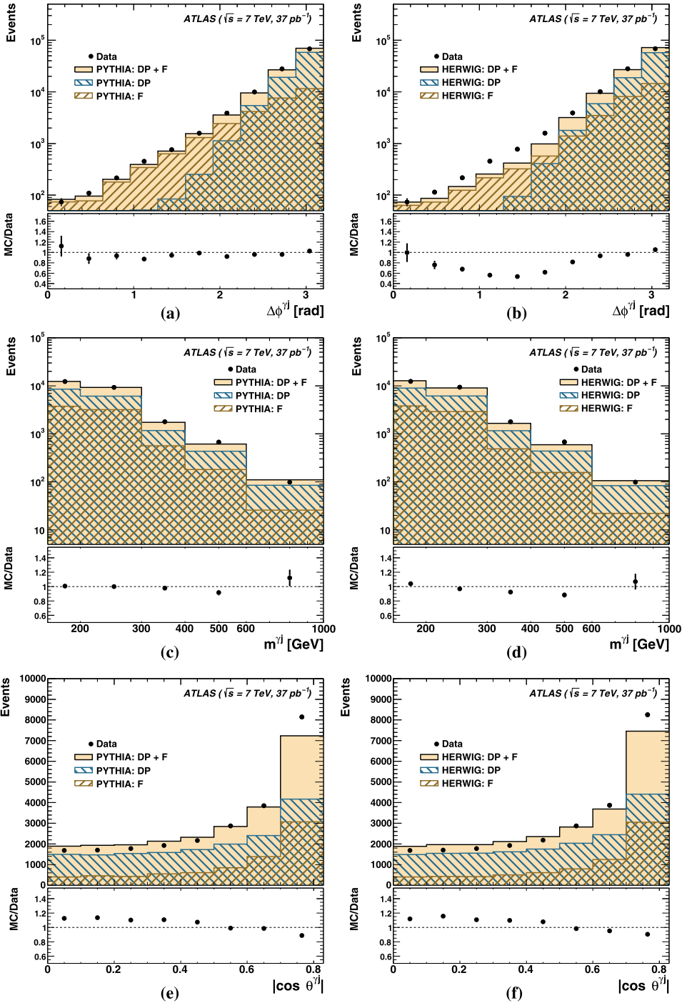
Fig. 4. The estimated signal yield in data (dots) using the signal leakage fractions from (a, c, e) PYTHIA or (b, d, f) HERWIG as functions of (a, b) \Delta\phi^j , (c, d) m^j and (e, f) |\cos\theta^j| . The distributions as functions of m^j ( |\cos\theta^j| ) include requirements on |\cos\theta^j| ( m^j ) and |\eta^\gamma + y^{\text{jet}}| (see text). Other details as in the caption to Fig. 3.
