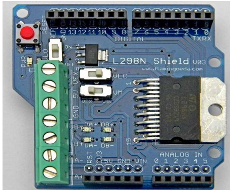
Gambar 2. Driver Motor L298
