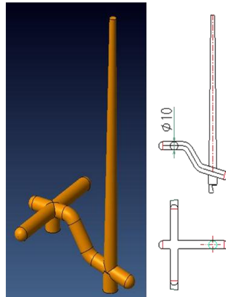
Gambar 10. Desain Runner .
