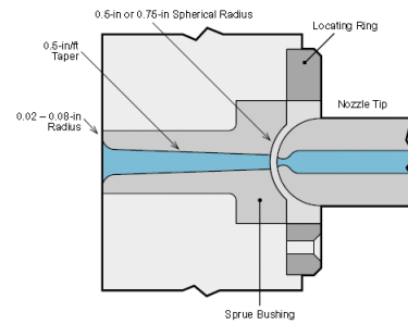
Gambar 4. Sprue Bushing
