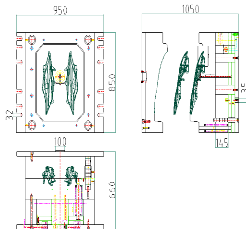
Gambar 8. Ukuran mold Cover Side 3/4
