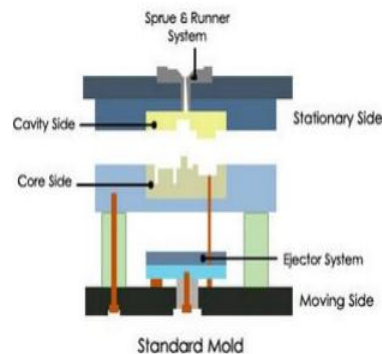
Gambar 1. Injection Molding.
