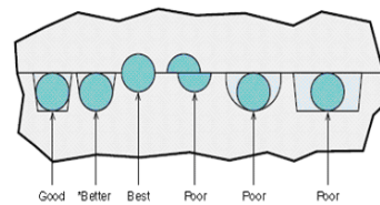
Gambar 5. Runner section
