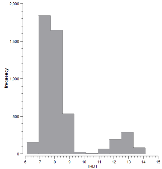
Figure 9. Distribution of THD-I
