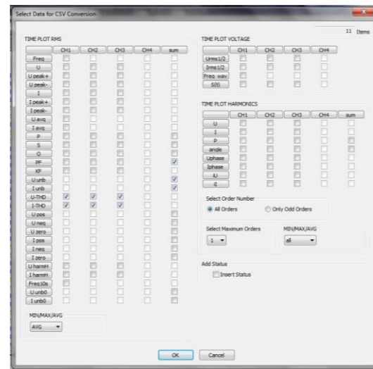
Figure 4. Transform the Data into CSV File
