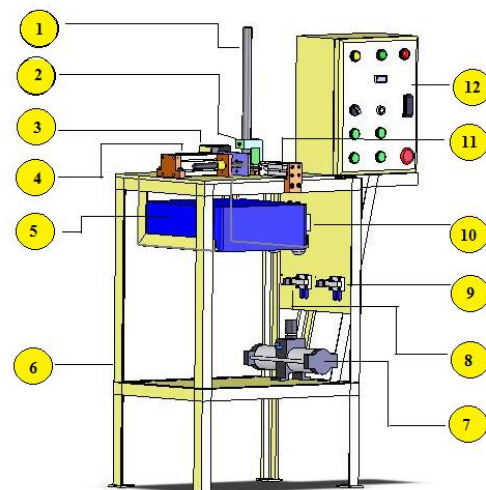
Gambar 5. Disain Mesin Caulking Guide Otomatis
