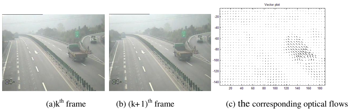
Fig.4 Optical flow field by H-S method
