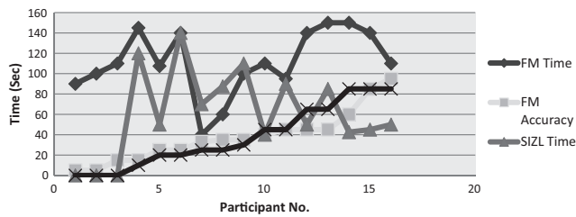
Fig. 5. Participants' time and accuracy when tested on both File Manager and SIZL.
