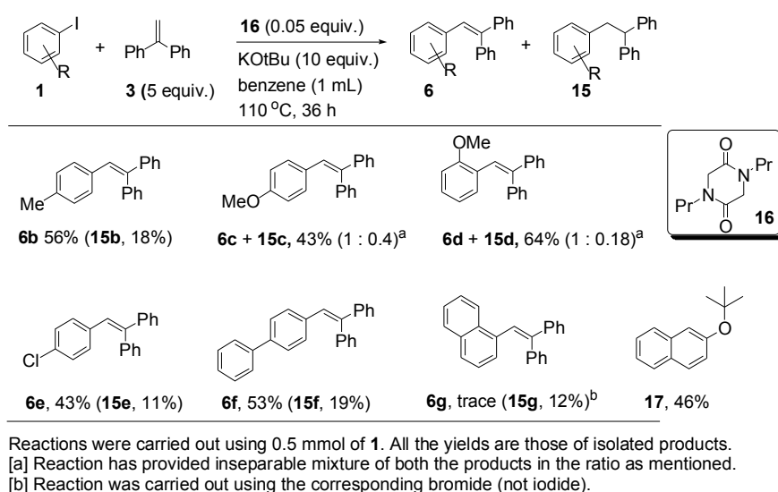
Figure 3. Scope of the formation of alkene products 6 .
