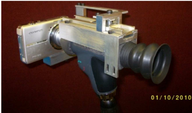
Figure 6. Panoptic monocular indirect ophthalmoscope (Welch-Allyn Inc., Skaneateles Falls, NY, USA) customised so to capture images with a wireless enabled digital camera. A cellphone then received these images for long-distance transmission.
