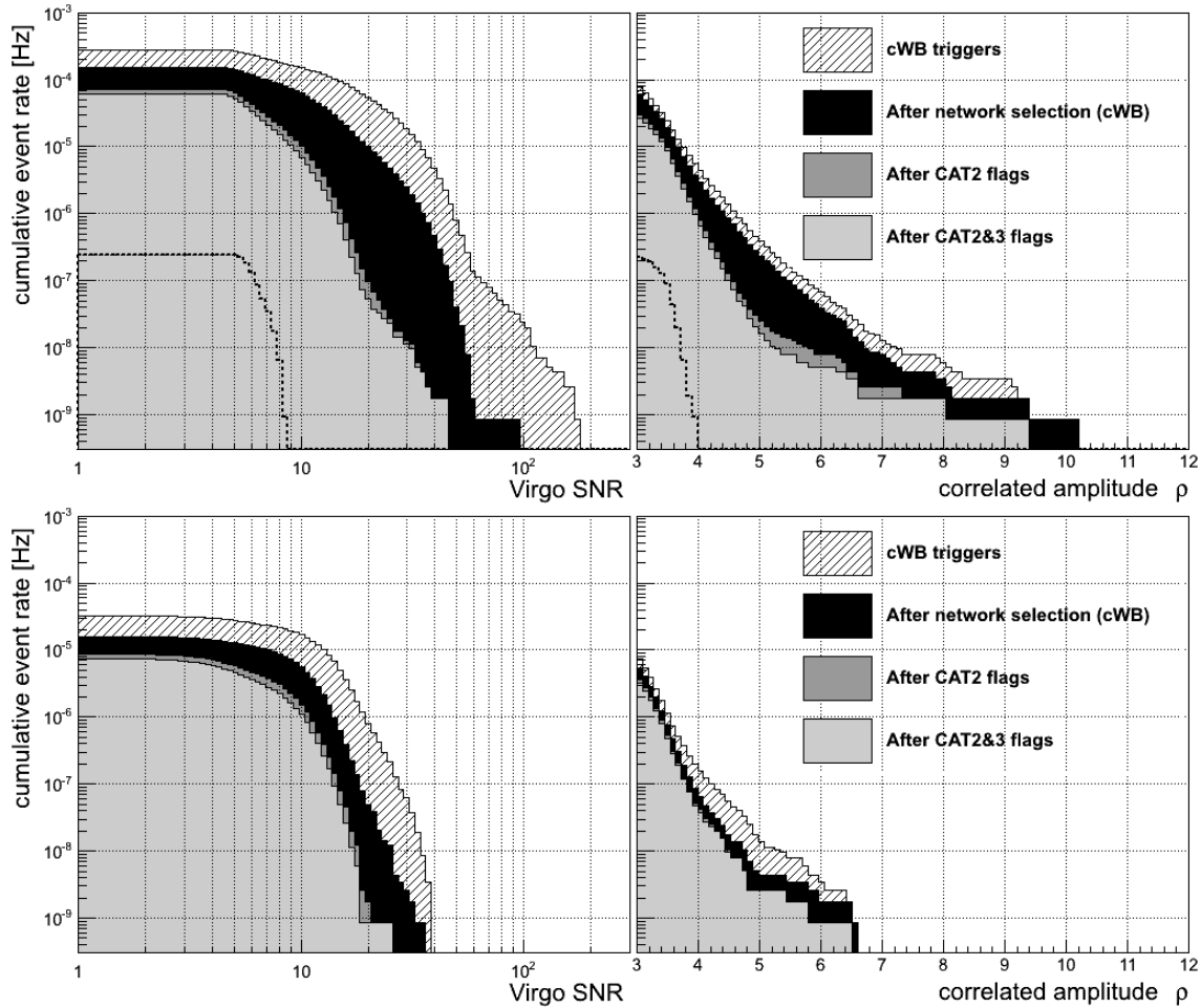
Figure 9. Effect of the Virgo DQ flags on burst-type (cWB) background triggers. Two months of VSR2 background data were considered and coherent LIGO-Virgo event distributions in double coincident time (upper row) and triple coincident time (lower row) are plotted. On the left, the distribution of Virgo SNR, which measures the Virgo contribution to the coherent data stream, is plotted and, on the right, events (with \rho > 3 ) are ranked with the correlated amplitude \rho . The hashed histograms show the trigger rate produced by cWB. When applying cWB selection cuts, it is possible to remove loud triggers, as shown by the black histograms. On top of this selection, applying CAT2 and CAT3 Virgo DQ flags allows for the reduction of the distribution tails even more. The distributions obtained with Gaussian noise are superimposed on double coincident time plots.
