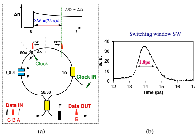
Fig. 3(a) Schematic diagram of TOAD; top -indication of all optically induced SOA index change \Delta n ; (b) TOAD measured switching window; ODL -optical delay line, OM -Sagnac loop optical midpoint, SOA - optical semiconductor amplifier, F -optical clock blocking filter, c - speed of light, SW -the width of the switching window
