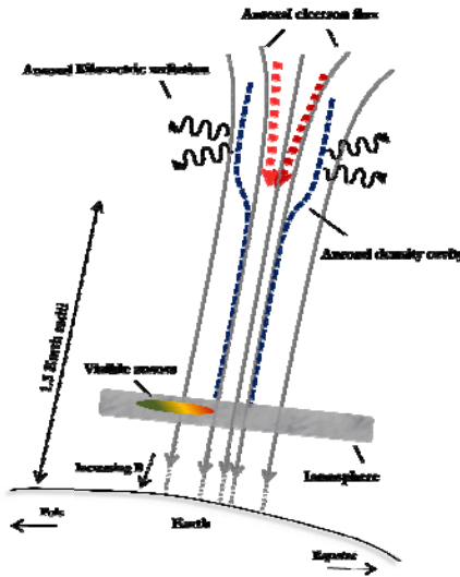
Figure 1: Representation of the AKR source region and terrestrial auroral process.
