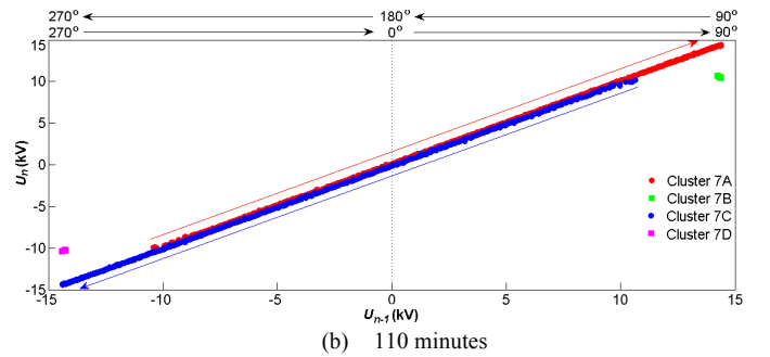
Fig. 3. The consecutive voltage plot, u_n vs u_{n-1} , of PD from a sample tested
