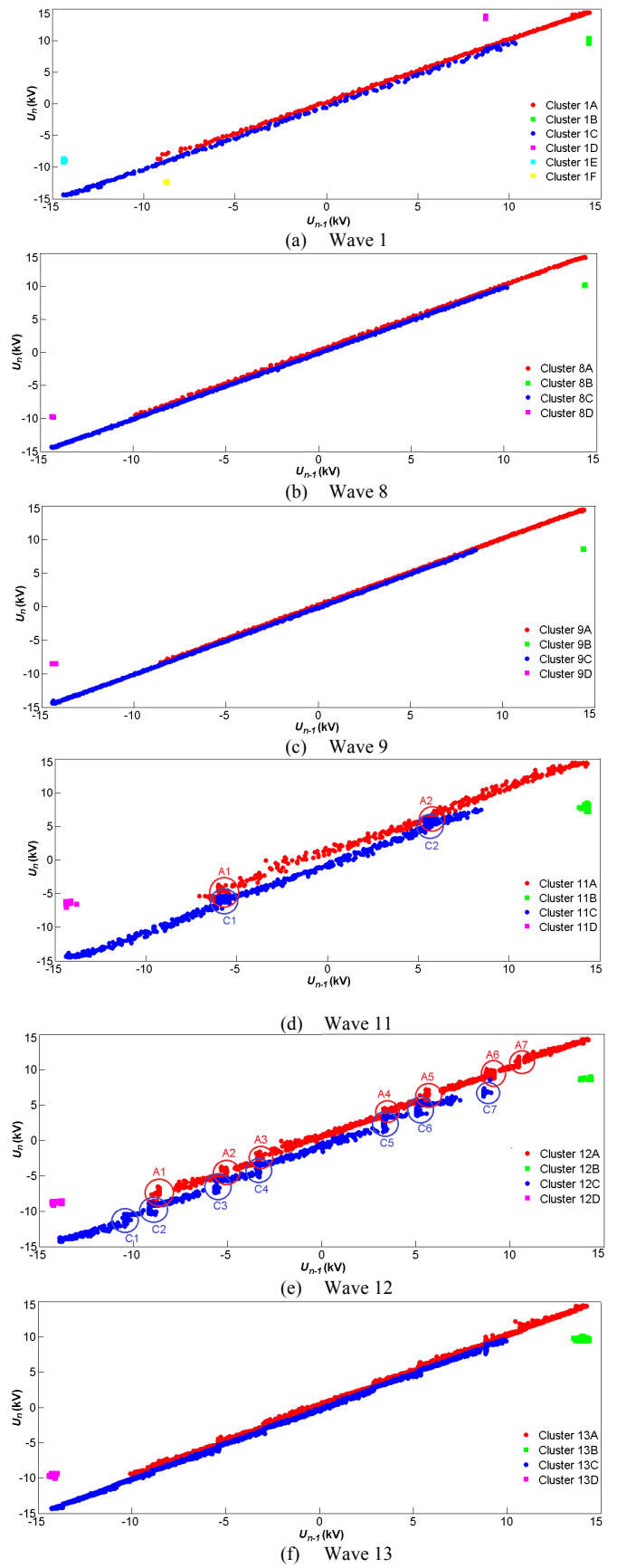
Fig. 5. The consecutive voltage plot, u_n vs u_{n-1} , of samples tested
