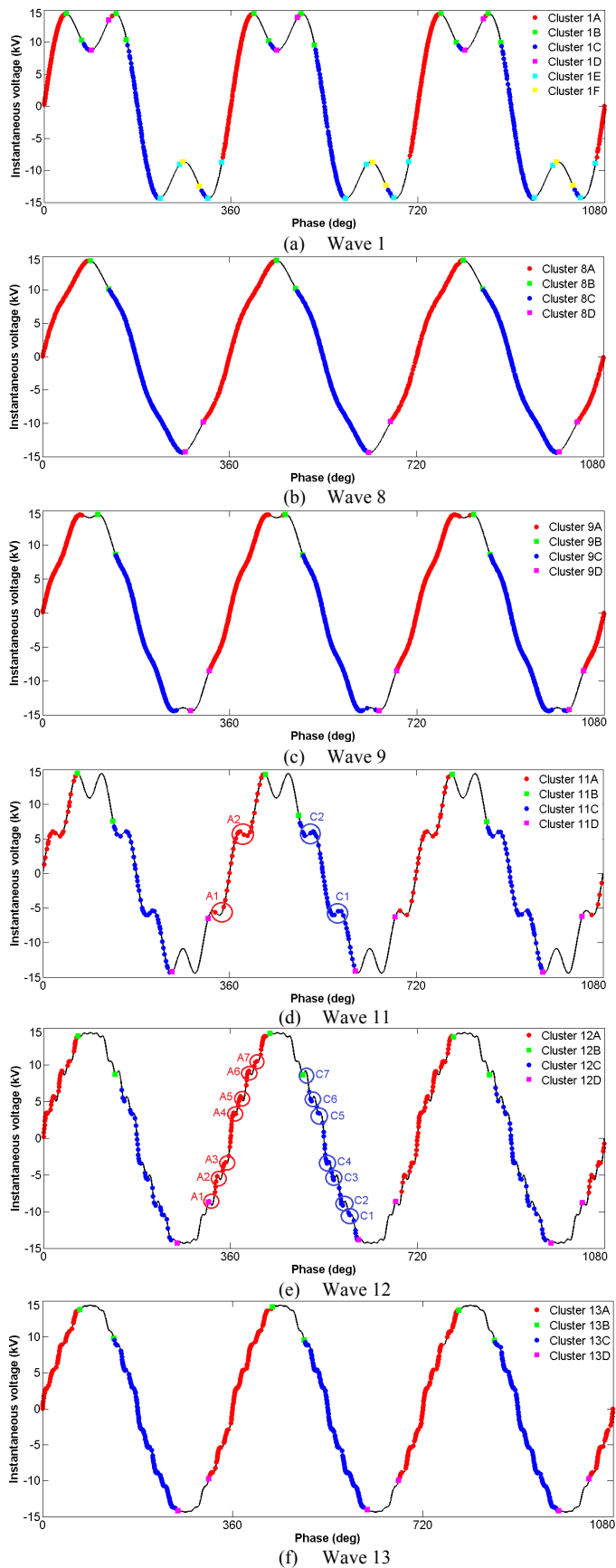
Fig. 4. The instantaneous voltage, u(t) , plot of samples tested
