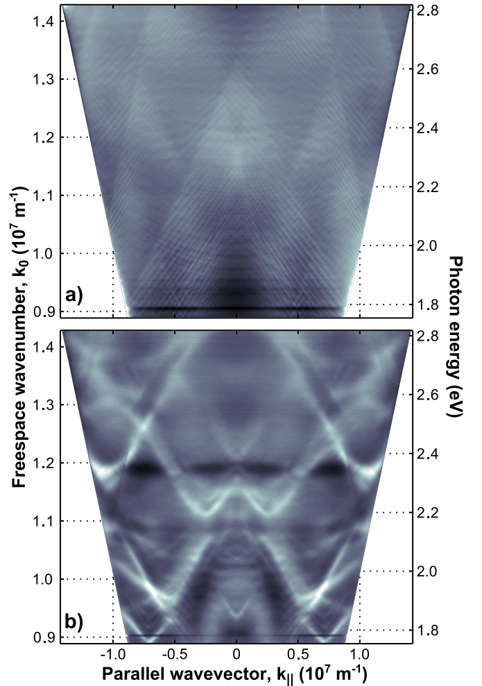
FIG. 3. Normalized k-space projection showing the angular PL intensity variation with frequency and inclinal angle along the \Gamma\mathbf{K}_a direction for the a) 850 nm and b) 4000 nm tall core-shell nanorods
