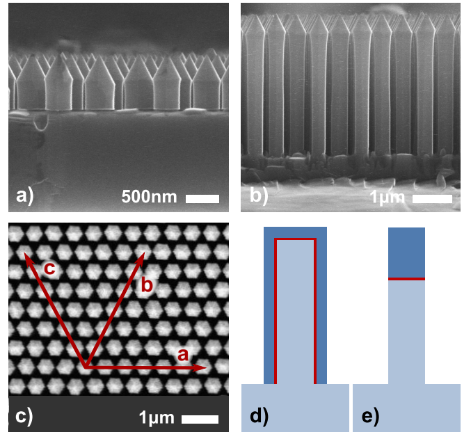
FIG. 1. Cross section of a) 850 nm and b) 4000 nm core-shell nanorods c) plan view of 4000 nm core-shell nanorods where the arrows indicate the lattice vectors. Schematic representation of d) core shell and e) quantum disc nanorod device configurations where red indicates the emitting region.
