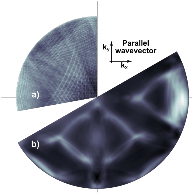
FIG. 4. Normalized in-plane k -space projection of angular PL showing the intensity variation with azimuth and inclinal angle for a single frequency at a) k_0 = 1.05 \times 10^7 \text{ m}^{-1} (2.07 eV) from the 850 nm tall core-shell nanorods and b) k_0 = 1.19 \times 10^7 \text{ m}^{-1} (2.34 eV) from the 4000 nm tall core-shell nanorods. k_x is parallel to the \Gamma\mathbf{K}_a direction.
