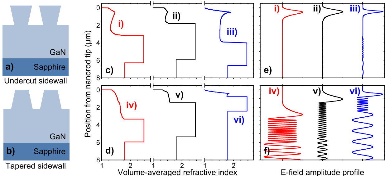
FIG. 6. Schematic representation of nanorod arrays with (a) undercut and (b) tapered sidewalls. Volume-averaged refractive index profiles (c,d) and modelled \mathbf{E} -field amplitude profile (e,f) of the first-order resonance in the PhC region for i) 3175 nm tall rods with undercut sidewalls (SQW4), ii) 1800 nm tall rods with undercut sidewalls (SQW2), iii) 4000 nm tall core-shell rods, iv) 3050 nm tall rods with tapered sidewalls (SQW3), v) 1700 nm tall rods with tapered sidewalls (SQW1) and vi) 850 nm tall core-shell rods.
