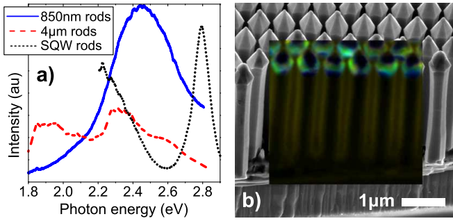
FIG. 2. a) PL spectra of core-shell (850 & 4000 nm high) and quantum disc (SQW) nanorods at normal incidence. b) (Color online) Real color representation of spatially resolved CL emission from 4000 nm core-shell nanorods.
