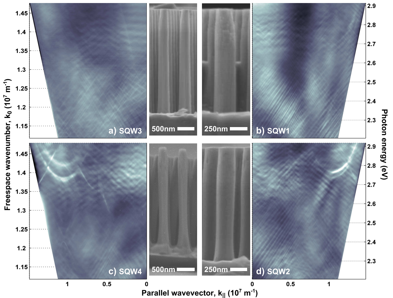
FIG. 5. Cross section SEM images and k-space projection of the angular PL intensity variation along the \Gamma\mathbf{K}_a direction for a) SQW3, tapered 3050 nm, b) SQW1 tapered 1700 nm, c) SQW4 undercut 3175 nm, d) SQW2 undercut 1800 nm high rods.
