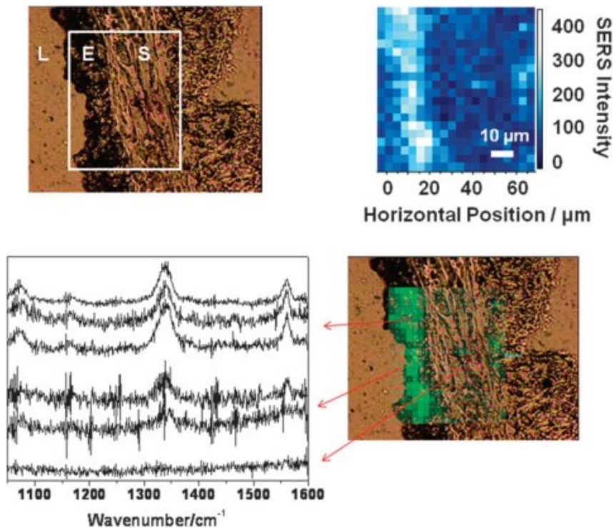
Figure 4: Detection of PSA ex vivo – top: bright field microscope image of a prostate tissue section. The grid shows the locations at which Raman spectra were acquired in a point mapping experiment. The false colour SERS image shows that the characteristic signal of the SERS-labelled antibody is observed selectively in the epithelium. Reproduced from [80] with permission from the PCCP Owner Societies.
