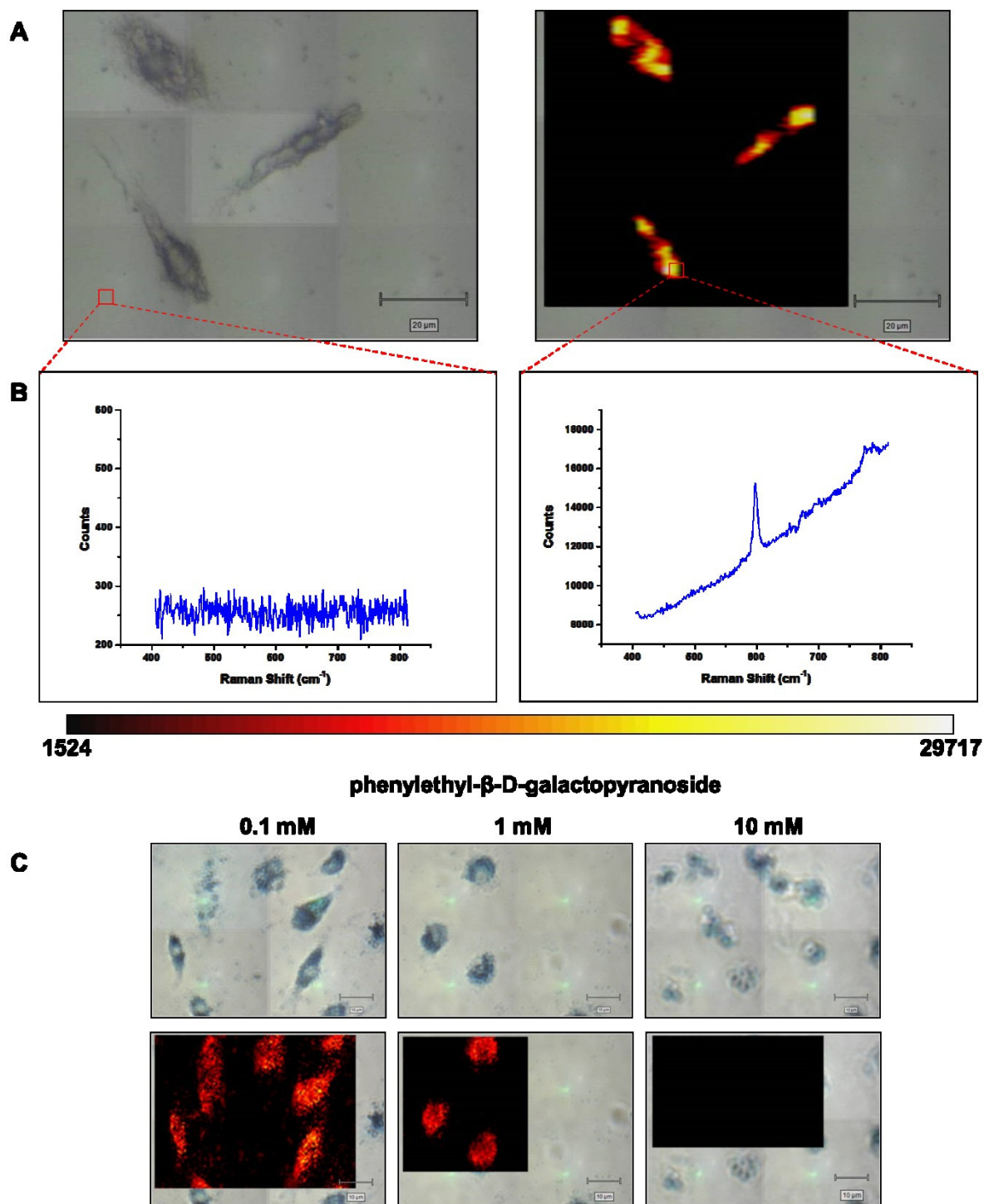
Figure 1: Intracellular conversion of X-Gal to the blue coloured product 5,5'-dibromo-4,4'-dichloro indigo by the enzyme \beta -galactosidase – A) white light and false colour image based on the 5,5'-dibromo-4,4'-dichloro indigo peak at 598\text{ cm}^{-1} , B) corresponding spectra from the highlighted areas and the associated false colour LUT bar and C) the effect of an enzyme inhibitor on the measured SERS signals. [62] Modified and reproduced by permission of the RSC.
