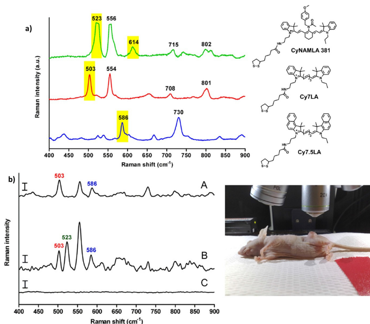
Figure 7: In vivo multiplex detection in xenograft tumour – a) Normalised SERS spectra of CyNAMLA-381, Cy7LA and Cy7.5LA after chemisorption of AuNPs and b) – A: SERS spectra from tumour site (peaks obtained at 503 and 586 cm -1 from two EGFR positive nanotags, Cy7LA and Cy7.5LA), B: SERS spectra from liver site (peaks obtained at 503, 523 and 586 cm -1 ) from two EGFR nanotag Cy7LA, Cy7.5 and anti-HER2 nanotag CyNAMLA-381 and C: SERS spectra from dorsal region. [105] Modified and reprinted with permission from Elsevier.
