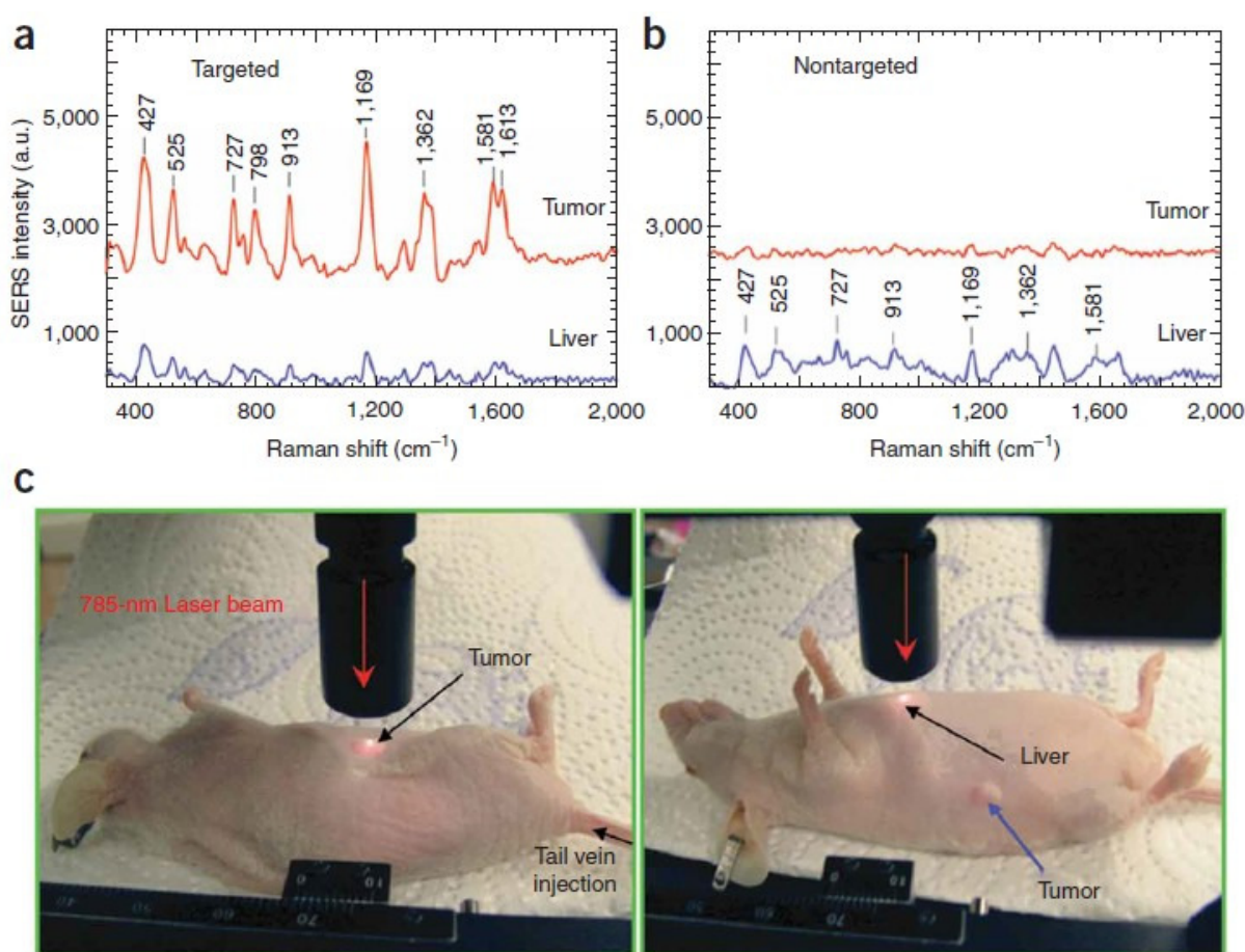
Figure 5: In vivo cancer targeting and surface enhanced Raman detection by using ScFv-antibody conjugated gold nanoparticles that recognise the tumour biomarker EGFR. (a,b) SERS spectra obtained from the tumour and the liver locations by using targeted (a) and nontargeted (b) nanoparticles. Two nude mice bearing human head-and-neck squamous cell carcinoma (Tu686) xenograft tumour (3-mm diameter) received 90 \mu L of ScFv EGFR-conjugated SERS tags or pegylated SERS tags (460 \mu M). The particles were administered via tail vein single injection. SERS spectra were taken 5 h after injection. (c) Photographs showing a laser beam focusing on
