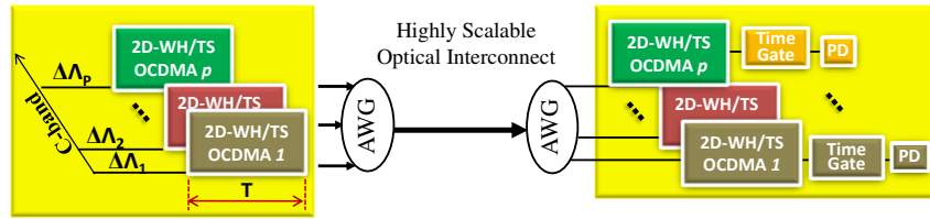
Figure 2. Conceptual diagram of a highly scalable optical interconnect. p 2D-WH/TS OCDMA subsystems broadcast over coarse C-WDM. Timing gates are used to suppress MAI: ( \Delta\lambda_i ) spectral band occupied by individual OCDMA subsystems, (PD) photodetector.
