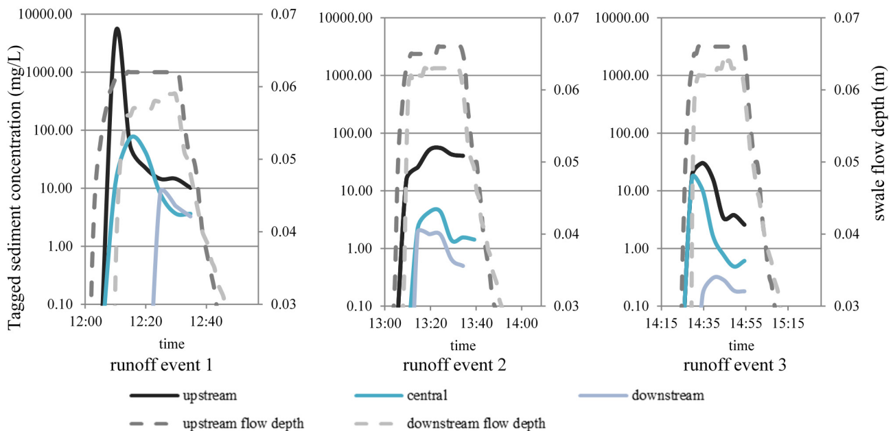
Figure 3. REO tagged sediment concentrations for artificial runoff events at the three surface runoff monitoring locations within the swale (upstream, central, and downstream locations)—Experiment 1 results.
