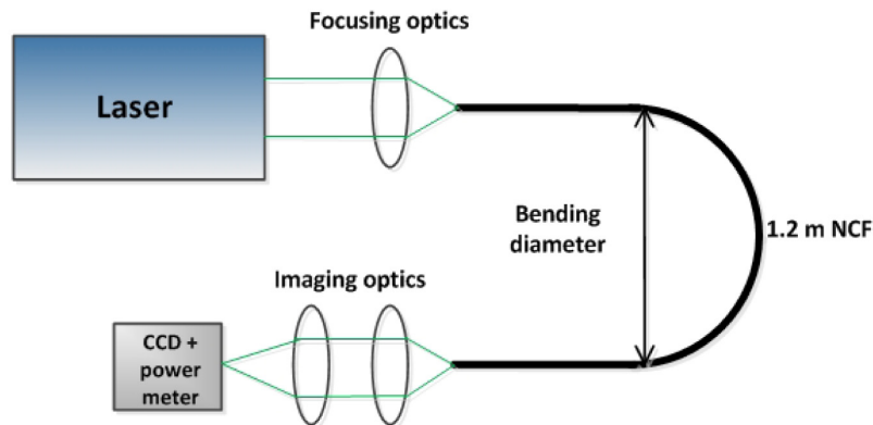
Fig. 4. Experimental setup for fiber bending tests.
