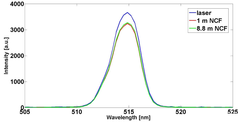
Fig. 8. Optical spectra of: picosecond laser beam (35 \mu J pulse energy, solid blue line); delivered beam through 1 m NCF (30 \mu J pulse energy, solid red line) and 8.8 m NCF (21.5 \mu J pulse energy, solid green line).
