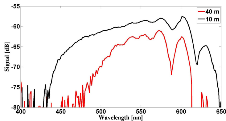
Fig. 2. Transmission spectra of 10 m (solid black line) and 40 m (solid red line) NCFs.
