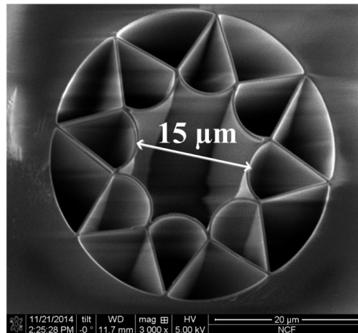
Fig. 1. SEM image of the fabricated NCF.
