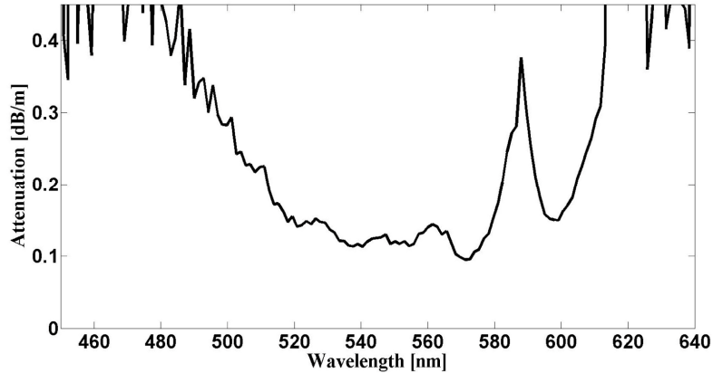
Fig. 3. Attenuation spectrum of the fabricated fiber.
