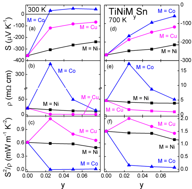
Figure 9. Composition dependence of the Seebeck coefficient ( S ), electrical resistivity ( \rho ), and thermoelectric power factor ( S^2/\rho ) for the \text{TiNiM}_y\text{Sn} ( M = \text{Co, Ni and Cu} ) series at (a–c) 300 and (d–f) 700 K.
