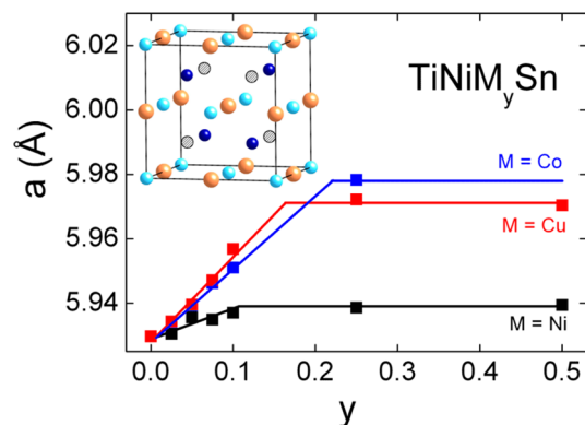
Figure 1. Lattice parameters of the HH phase for the \text{TiNiM}_y\text{Sn} ( M = \text{Co} , \text{Ni} and \text{Cu} ) series. The inset shows the HH unit cell with Ti (pale blue), Ni (dark blue) and Sn (gold) sublattices. Ni occupies the Y1 sites. The other tetrahedral sites (Y2), indicated as hatched spheres, are occupied in the FH structure.
