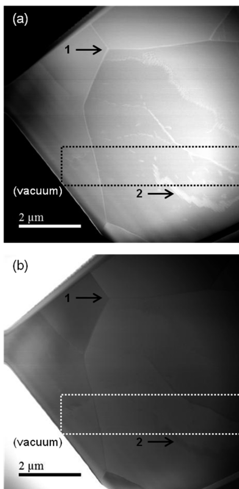
Figure 5. (a) Dark-field and (b) bright-field STEM images of a wide-area cross-section through a TiNi 1.05 Sn pellet. In both images, the contrast is largely uniform, and there is no evidence for clear phase segregation or the formation of inclusions. Continuous bright lines in the dark field image, such as the triple boundary indicated at position 1, are the boundaries and junctions between separate grains, which have fused. Weaker features such as those indicated at position 2 are consistent with dislocation networks. The rectangular section is prepared by FIB techniques and the thin protective layer of Pt that was deposited prior to ion milling is just visible to the lower right. The dotted lines indicate the region used for EDX spectrum imaging.
