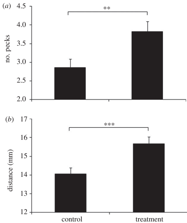
Figure 1. (a) Mean \pm s.e. number of pecks needed to successfully catch interference-coloured (treatment) and non-interference-coloured (control) stimuli. (b) Mean \pm s.e. distance of unsuccessful pecks at treatment and control stimuli, measured in mm from the centre of the prey item at the time of pecking. ** p < 0.01 ; *** p < 0.001 .
