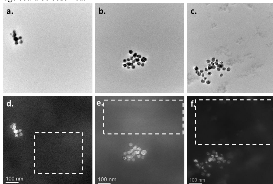
Figure 1. EFTEM analysis of Ag NPs in 200 (a) and (d) (Sample A), 500 (b) and (e) (Sample B), and 2000 fold (c) and (f) (Sample C) with BF TEM images a.)-c.) and thickness maps d.)-f.);dashed boxes indicates typical areas of t/\lambda mean values measurement .
