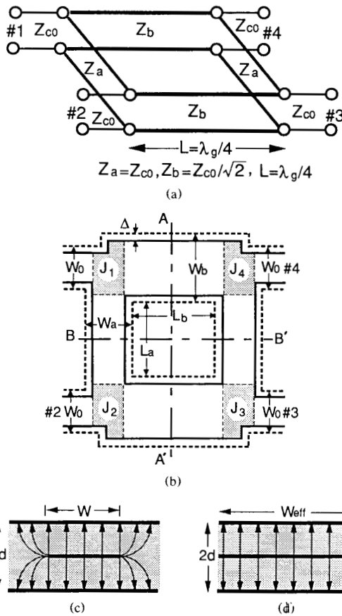
Fig. 1. Branch-line 3 dB hybrid circuit model. (a) Transmission line circuit model. (b) Planar-type 3 dB hybrid model. (c) Triplate stripline. (d) Planar-type transmission line model ( W_{eff} = W + 2\Delta , \Delta = (2/\pi)d \cdot \ln 2 ).
