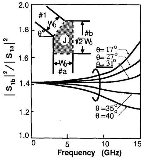
Fig. 6. Frequency characteristics of three-port junction with the connecting angle \theta as a parameter.
