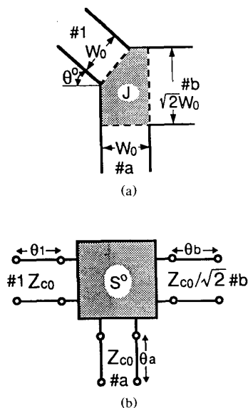
Fig. 3. Three-port planar junction and its equivalent circuit. (a) Circuit designed to satisfy the relation |S_{ij}| = |S_{ij}^0| . (b) Equivalent circuit of (a).
