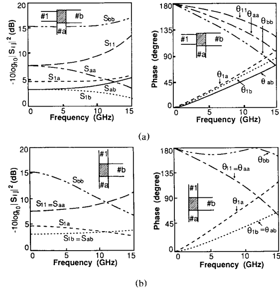
Fig. 5. Frequency characteristics of rectangular junction circuit. (a) Horizontal connection ( \theta = 0^\circ ). (b) Vertical connection ( \theta = 90^\circ ).
