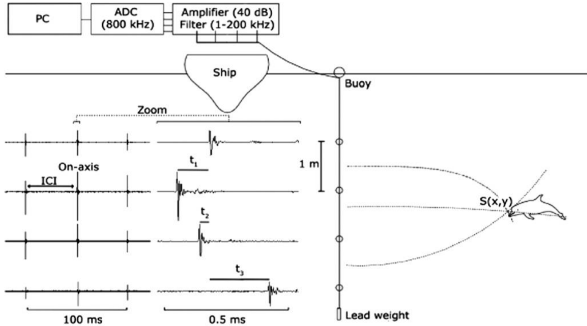
Figure 1. Setup for recordings of Tursiops aduncus . The recording setup t1, t2, and t3 are the time-of-arrival differences between the same click arriving on the four different hydrophones.
