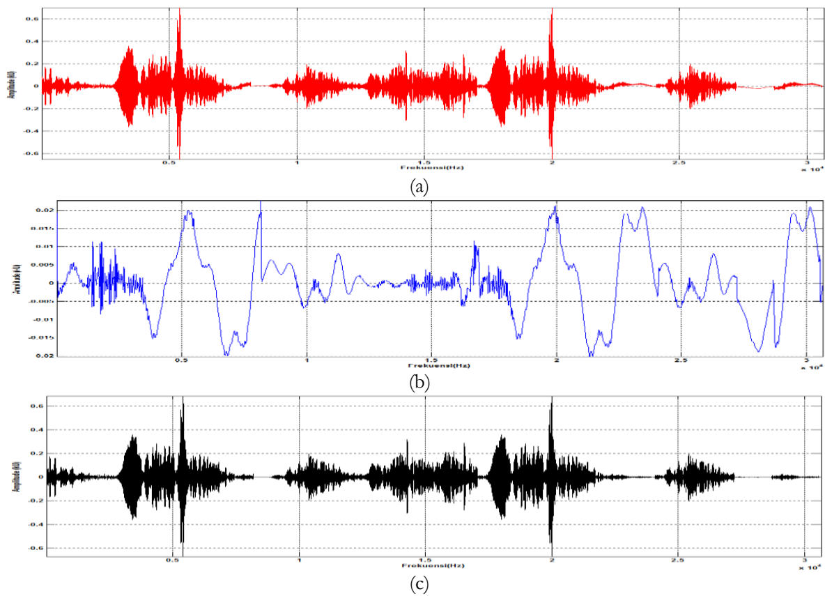
Figure 7. Signal of whistle 3 (a) original signal, (b) denoised signal, (c) residual signal using Haar wavelet
