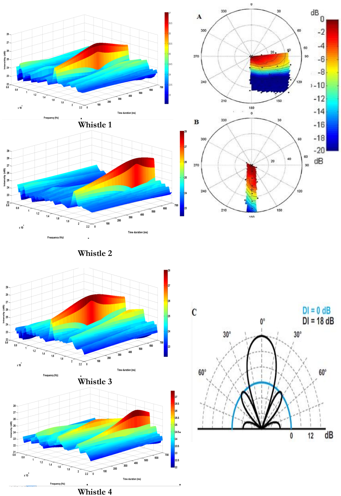
Figure 10. 3D figure (Intensity, Frequency, and Time duration ) whistle 1,2,3,and 4 with approach 4 type signal in beam pattern (A, B), beampattern from an omni directional sound source (C).
