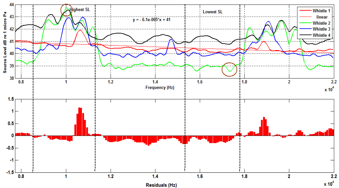
Figure 9. Source Level (SL) of whistle 1, 2,3, and 4.
