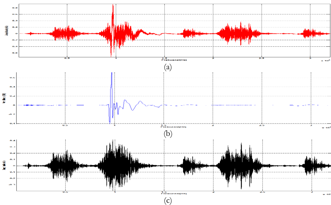
Figure 6. Signal of whistle 2 (a) original signal, (b) denoised signal, (c) residual signal using Haar wavelet
