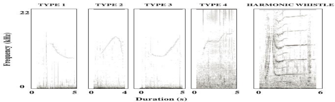
Figure 2. Spectrograms of the five sound whistle types (type 1, type 2, type 3, type 4, and harmonic) of Risso's dolphins (with sampling rate: 44100 Hz, -10 db, FFT 512).
