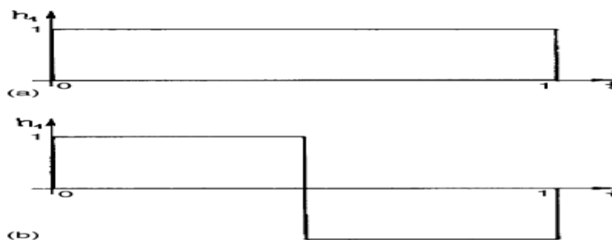
Figure 3. Haar wavelet: (a) scaling function, (b) mother wavelet.
