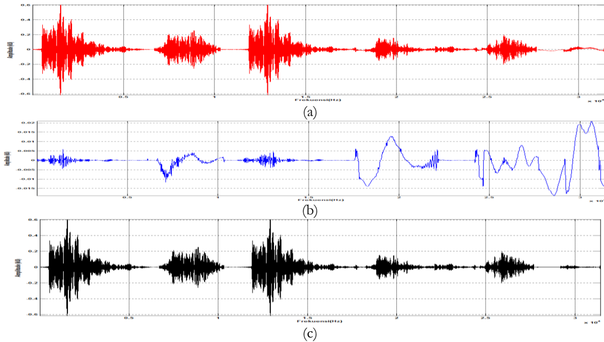
Figure 8. Signal of whistle 4 (a) original signal, (b) denoised signal, (c) residual signal using Haar wavelet
