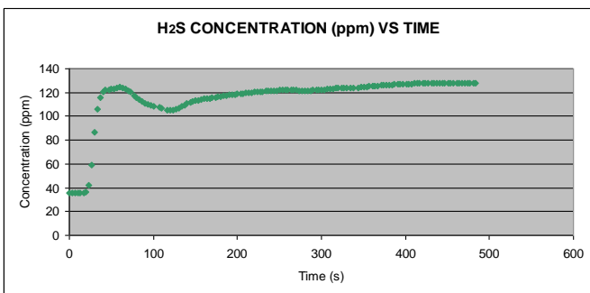
Figure 20. H 2 S Concentration Relative to Time
