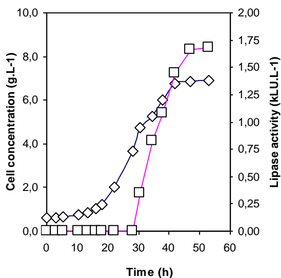
Figure 4. Profile of lipase production in 10 g L -1 palm cooking oil ( pH=6.0, T= 30° C, Aeration = 1 vvm, Agitation = 500 rpm )
