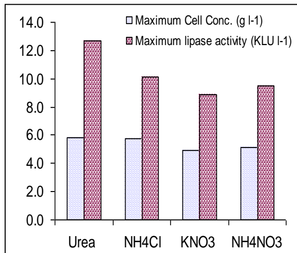
Figure 6. Effect of nitrogen sources on lipase production ( pH=6.0, T= 30° C, Aeration = 1 vvm, Agitation = 500 rpm and palm oil = 10 g L -1 )
