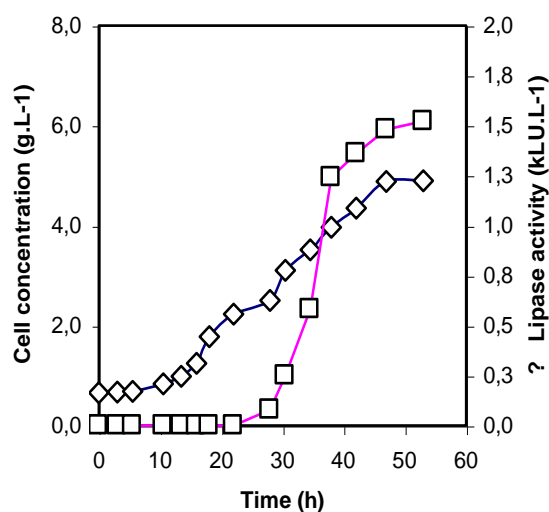
Figure 1. Profile of lipase production in 10 \text{ g L}^{-1} palmitic acid ( \text{pH}=6.0 , T= 30^\circ \text{ C} , Aeration = 1 vvm, Agitation = 500 rpm )
