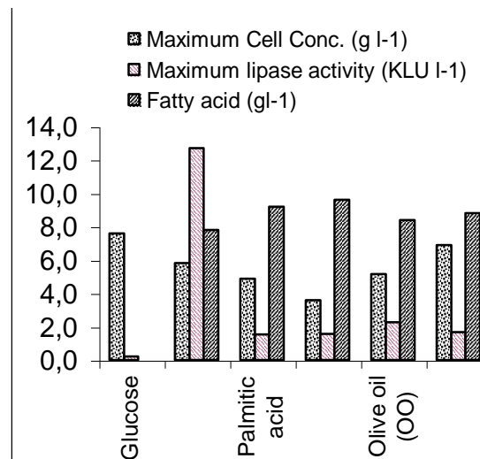
Figure 5. Effect of lipase production on different substrates ( pH=6.0, T= 30° C, Aeration = 1 vvm, Agitation = 500 rpm and cooking oil = 10
