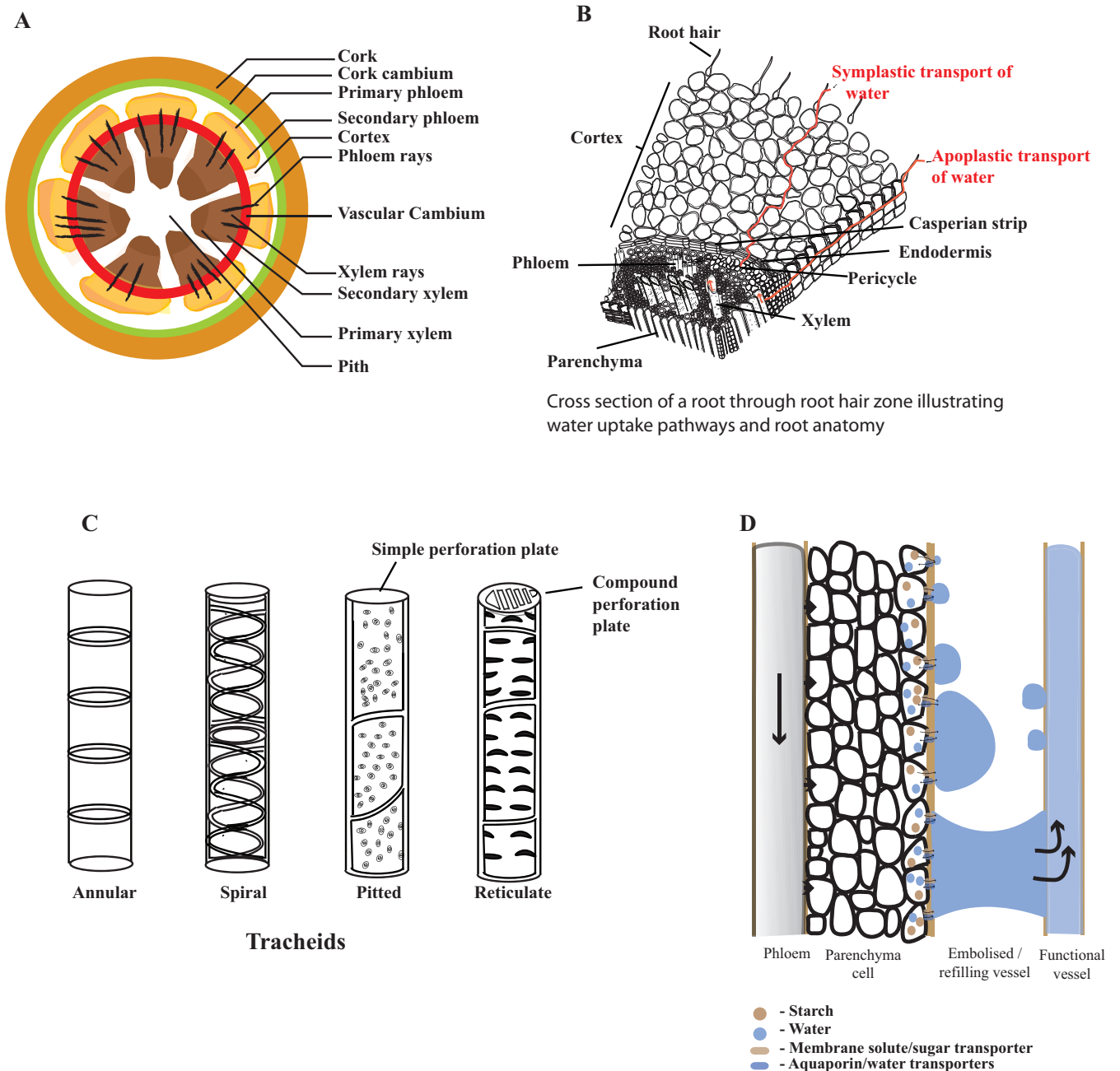
Figure 1: Morphology related to water transport in plants. A. Cross-section of a typical wood stem. The parts relevant to water transport are labeled. B. Water transport pathways through root hair. Red lines show both the symplastic and apoplastic routes of water transport through roots. C. Diversity of tracheid types. The morphology of the internal walls of tracheids influences the transport of water through the tracheid. D. Brodersen et al's (2010) proposed mechanism for embolism repair. According to this model, embolisms cause neighboring cells to release solutes into the affected vessel. The resulting osmotic gradient causes water movement from surrounding fibers and cells into the vessel. Eventually, the water droplets span the whole width of the vessel. Because the water in all vessels, including neighboring ones, is under a state of negative pressure, these water droplets may move to neighboring vessels, keeping the embolism in place. If however, there is net water accumulation within the embolised vessel, and the gas present in that vessel will eventually dissolve to repair the embolism (Brodersen et al., 2010).
