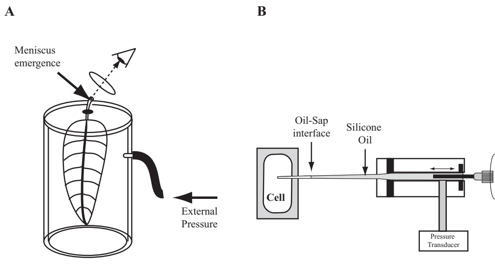
Figure 2: Techniques of pressure measurements in plants. A. Scholander pressure chamber method: Originally based on a previous method used by Dixon and Joly (1900), the Scholander pressure chamber method was the first to successfully demonstrate and measure negative sap pressures in plants. However, they are invasive and error-prone due to the requirement that the plant leaf or twig be detached from the plant for the purpose of the experiment. B. Pressure microprobe technique: A fairly non-invasive technique to measure the internal pressures in plant xylem without significantly altering its structure. It is sensitive at considerably lower range of pressures than the Scholander technique. It is also relatively more difficult to position within a plant tissue.
