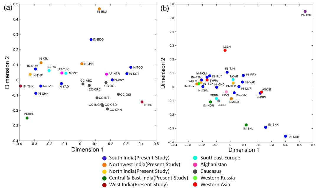
Figure 3. Multidimensional scaling (MDS) plot based on Rst values of Y-STRs for haplogroups (a) J2a-M410 and (b) J2b-M102. Dots represent different populations worldwide. CC = Caucasian, IN = Indian, AF = Afghanistani, ABZ = Abkhaz, BDG = Baduga, BNJ = Banjara, BHL = Bahelia, CHN = Chechen (Chechnya), DG = Chechen (Dagestan), INT = Chechen Ingushetia, CHN = Chenchu, CRC = Circassians, HVK = Havik, HZR = Hazara, ING = Ingush, KBJ = Kamboj, KOT = Kota, LHN = Lohana, MK = Mahadev Koli, MONT = Montenegrin, OSD = Ossets (Digor), OSI = Ossets (Iron), NOM = Indian Nomads (Pichakuntla & Mondli), SERB = Serbian, TJK = Tajik, THK = Thakar, THP = Thapa, TOD = Toda, VNY = Vanniyar, YAD = Yadav, IRAN = Iranian, LEBN = Lebanese, MONT = Montenegrin, SERB = Serbian, SYRIA = Syrian, WRUS = WesternRussia, CCSS = Caucasus, ASR = Asur, BHL = Bahelia, BUX = Buxas, CND = CapeNadar, CHN = Chenchu, EZH = Ezhava, KOR = Korku, MVR = Maravar, MNA = Meena, NKR = Narikuravar, PLY = Paliyan, PRV = Paravar, PRY = Parayar, NOM = Indian Nomads (Pichakuntla & Mondli), SHK = Shikari, TDV = Tadvi, TJN = Tamil Jains, THP = Thapa, VNY = Vanniyar, VAD = Yadhava, ASKNZ = Ashkenazi.
