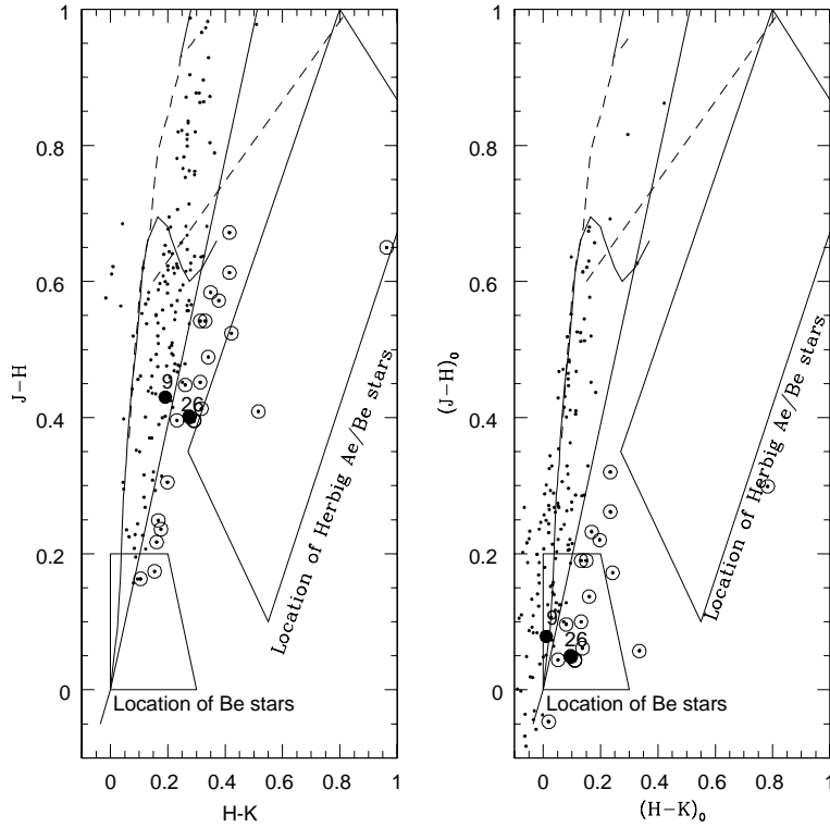
Figure 13. NIR colour-colour diagram for the cluster Be 86. Symbols and panels have the same meaning as in Fig. 1.
