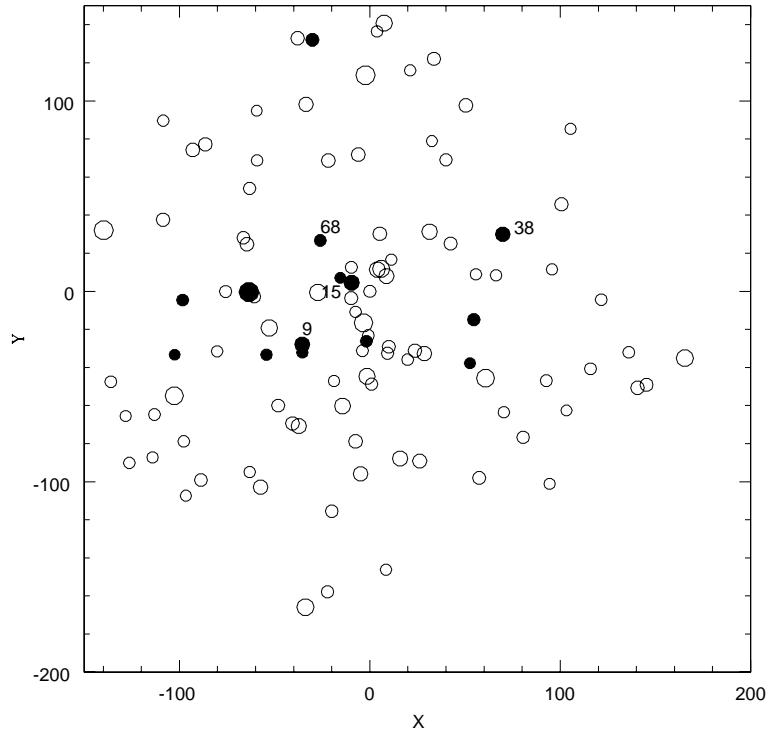
Figure 9. Cluster field of Be87 showing pre-MS stars and normal stars separately. The symbols have the same meaning as in Fig. 3.
