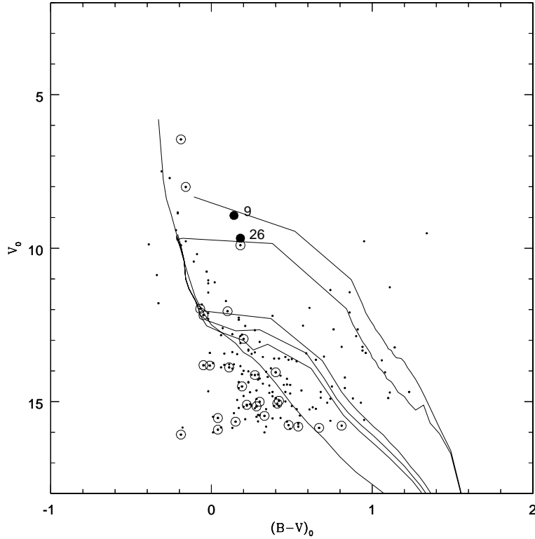
Figure 14. Pre-MS isochrone fittings for the cluster Be 86. The isochrones for the ages, 0.25, 0.5, 5, 7.5 and 10 Myr are shown.
