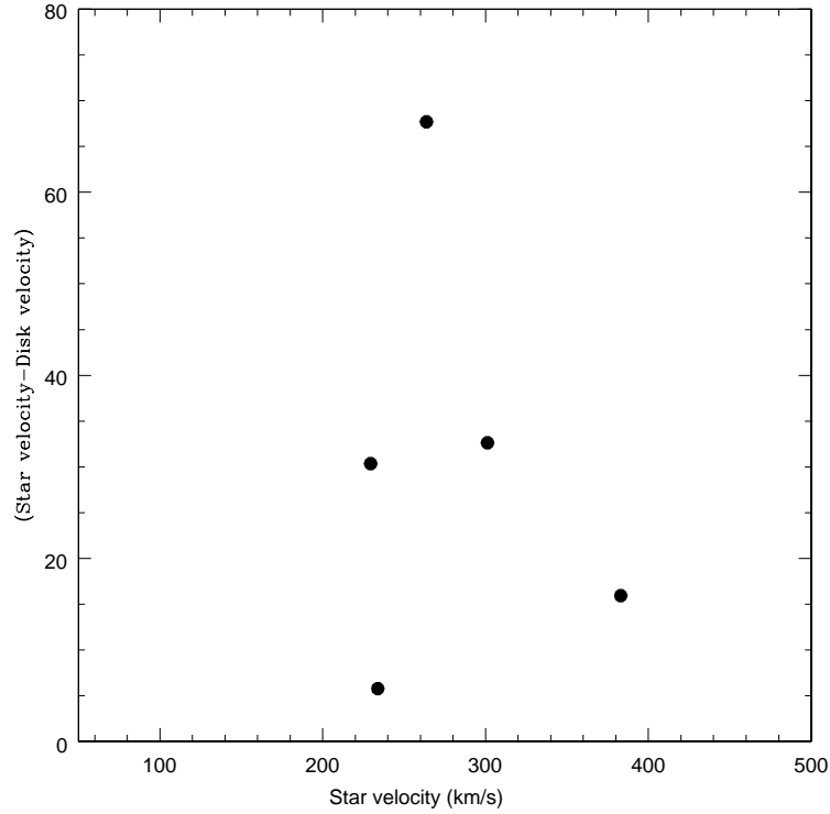
Figure 19. The relative rotational velocity between the star and its disk is plotted against the rotational velocity of the star. The velocities are plotted for the emission stars Be 87(38), NGC 6910 (26), Be 87(15), IC 4996(23) and Be 86(9), in the order of increasing stellar rotational velocity.
