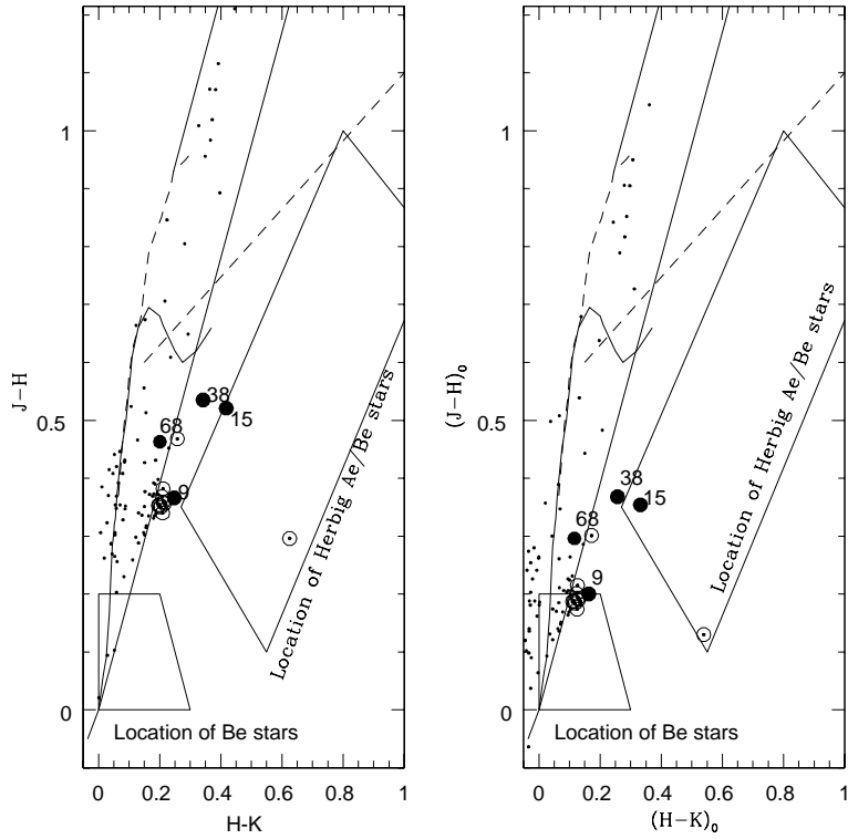
Figure 7. NIR colour-colour diagram of the cluster, Be 87. Symbols and panels have the same meaning as in Fig. 1.
