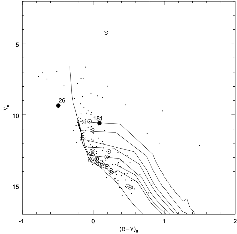
Figure 5. Pre-MS isochrone fittings for the cluster NGC 6910. The isochrones for the ages 0.5, 1, 2, 3, 5, 7.5 and 10 Myr are shown.
