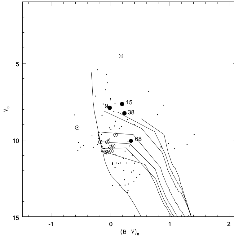
Figure 8. Pre-MS isochrone fittings for the CMD of the cluster Be 87. The isochrones for the ages, 0.15, 0.2, 0.25, 0.5, 1, 1.5 and 2 Myr are shown.
