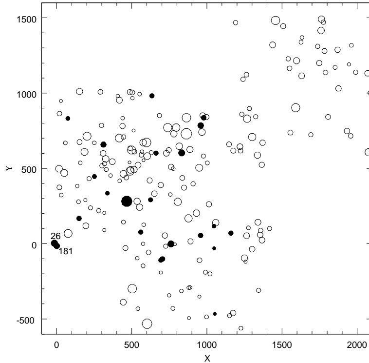
Figure 6. Cluster field of NGC 6910 showing pre-MS stars and normal stars separately. The symbols have the same meaning as in Fig. 3.
