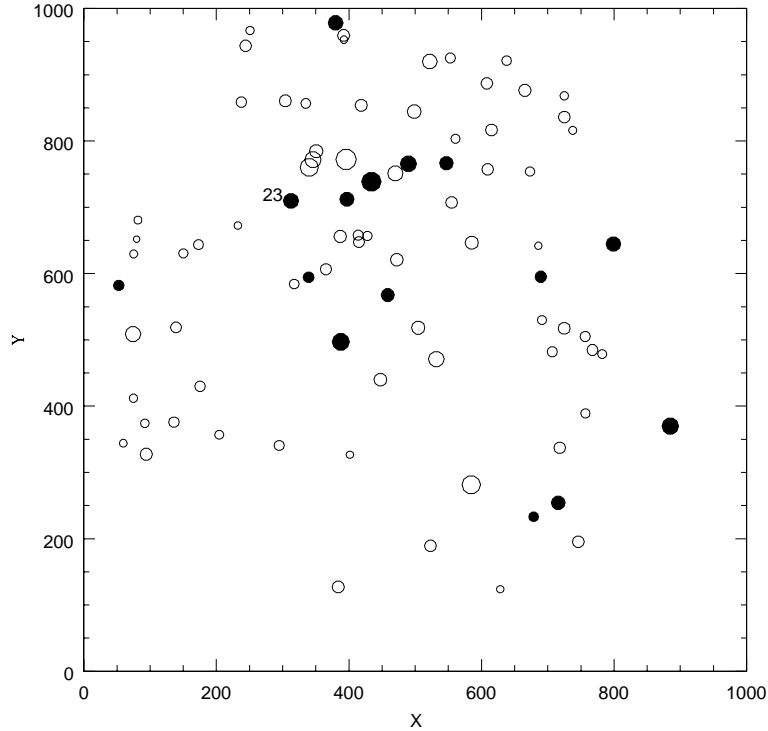
Figure 3. Cluster field of IC 4996 showing pre-MS stars and normal stars separately. Normal stars are shown as open circles, pre-MS stars are shown as filled circles and the emission stars are shown as labeled filled circles.
