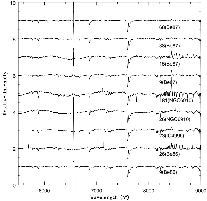
Figure 17. Flux calibrated, normalised, continuum fitted spectra of 9 Be stars in red region.
