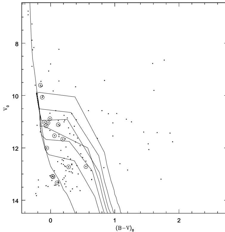
Figure 11. Pre-MS isochrone fittings for the cluster Biurakan 2. Isochrones for ages 0.5, 1, 1.5, 2, 3 and 5 Myr are shown.
