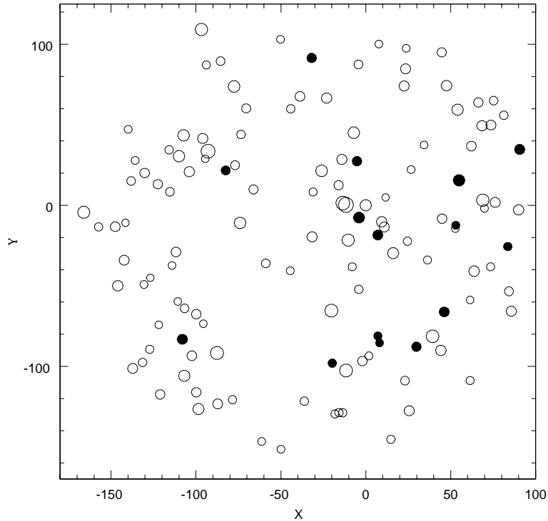
Figure 12. Cluster field of Biurakan 2 showing pre-MS stars and normal stars separately. The symbols have the same meaning as in Fig. 3.
