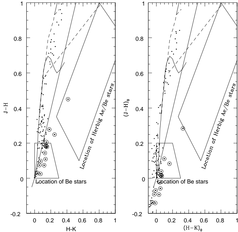
Figure 10. NIR colour-colour diagram for the cluster Biurakan 2. Symbols and panels have the same meaning as in Fig. 1.
