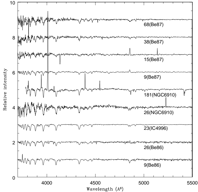
Figure 16. Flux calibrated, normalised, continuum fitted spectra of 9 Be stars in blue region.
