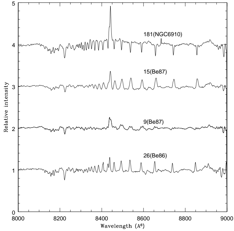
Figure 18. Spectra showing 3 stars with emission lines and 1 star with absorption lines in red end of the optical spectrum.
