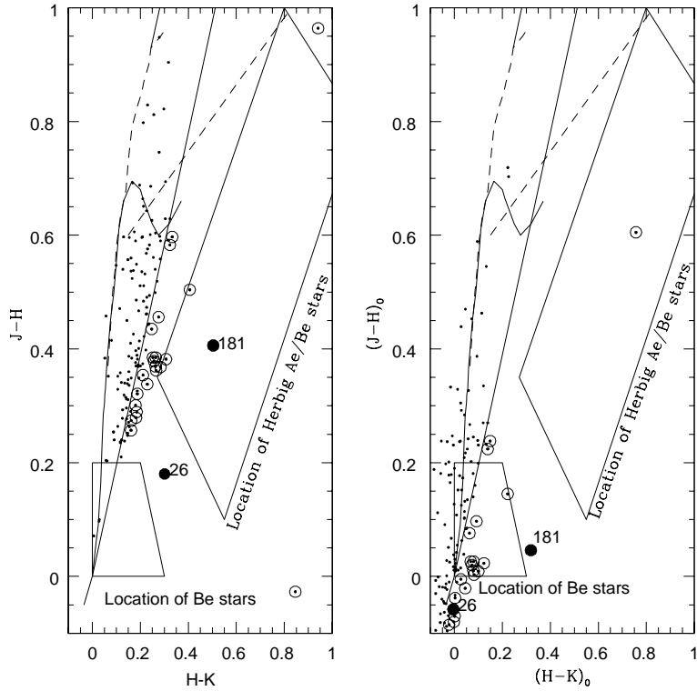
Figure 4. NIR colour-colour diagram for the cluster NGC 6910. Symbols and panels have the same meaning as in Fig. 1.
