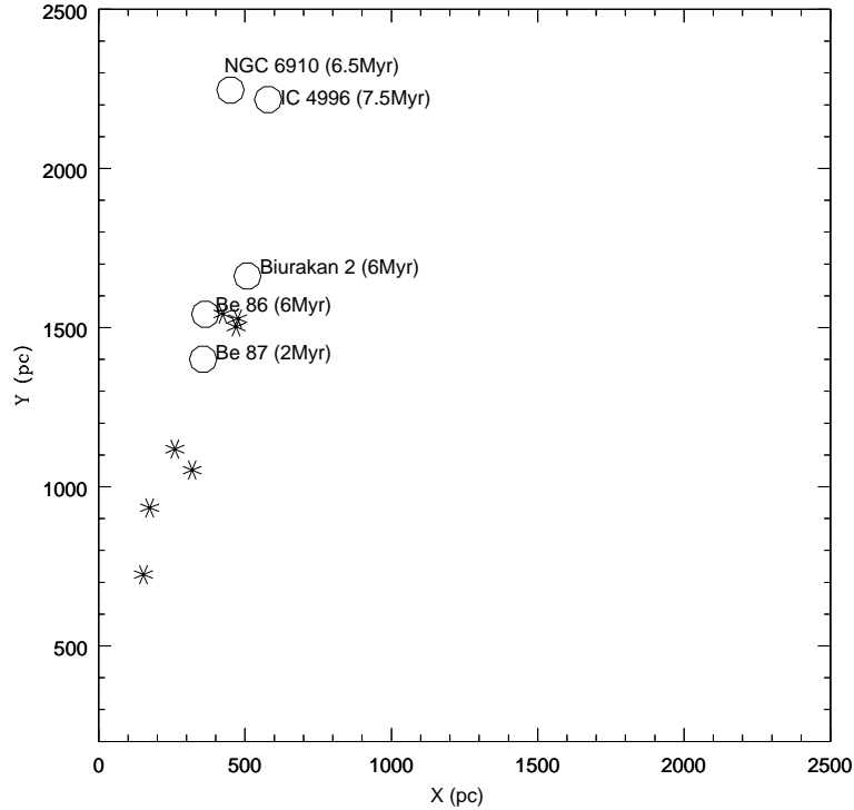
Figure 20. Location of clusters in the Cygnus region. The labeled open circles along with their turn-off ages, indicate clusters studied here. The asterisks indicate clusters present in the region, but not studied here.
