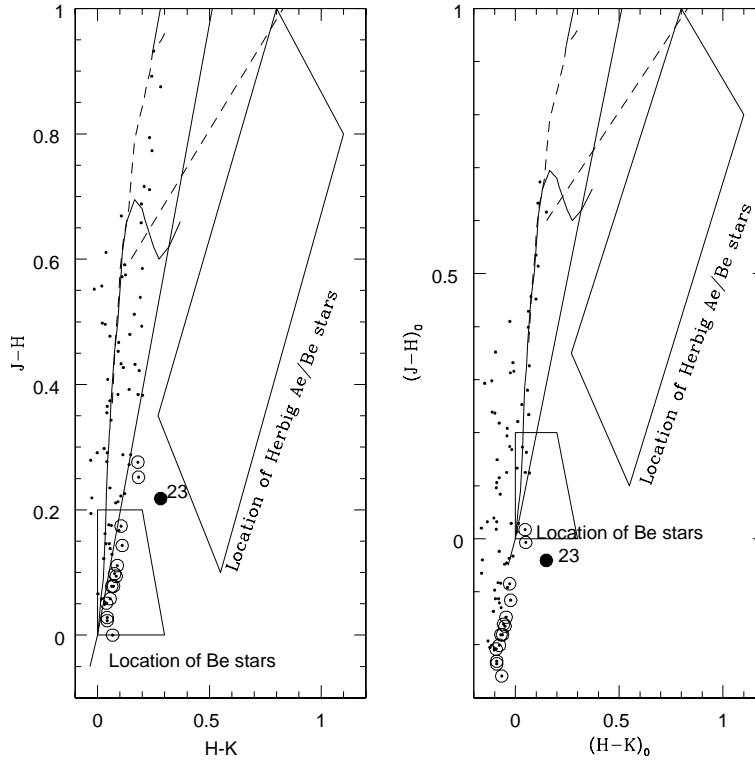
Figure 1. NIR colour-colour diagram for the cluster IC 4996. Dots indicate normal stars. Encircled dots indicate pre-MS stars. Stars with H_{\alpha} emission are shown as labeled and filled circle. The left panel shows colours uncorrected for reddening, whereas the right panel shows colours corrected for reddening. The reddening value as estimated from the ZAMS fitting is used for NIR dereddening, using the relation in Bessell & Brett (1988).
