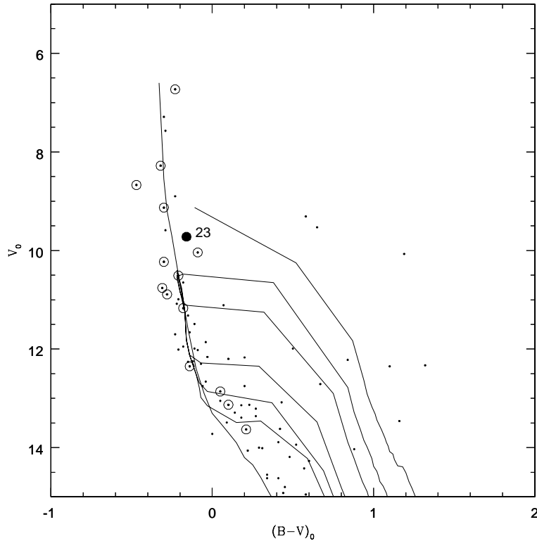
Figure 2. Pre-MS isochrone fittings for the cluster IC 4996. The isochrones for the ages 0.25, 0.5, 1, 3, 5 and 7 Myr are shown.
