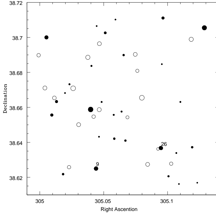
Figure 15. Cluster field of Be 86 showing pre-MS stars and normal stars separately. The symbols have the same meaning as in Fig. 3.
