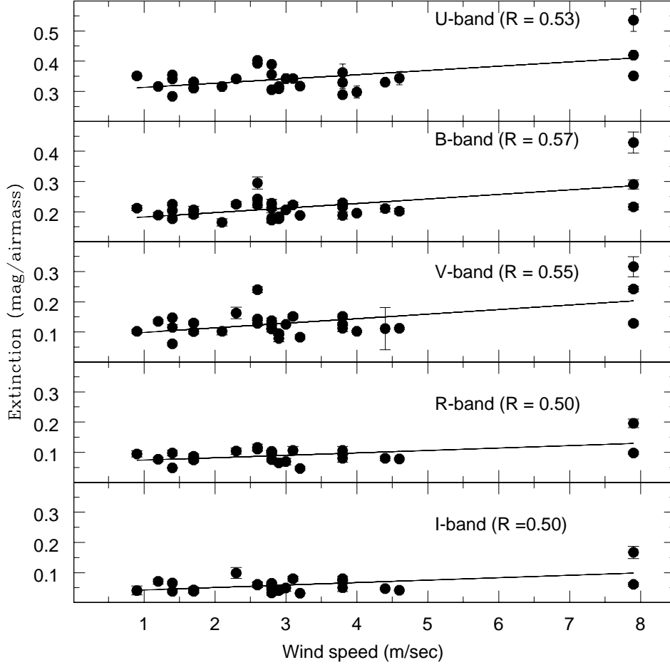
Figure 3. Variation of extinction in UBVRI passbands with the average night time wind speed. The linear correlation coefficient in each band is given in the respective panel. The error bars when not visible are smaller than the symbol size. The solid line is the unweighted linear least squares fit to the data.
