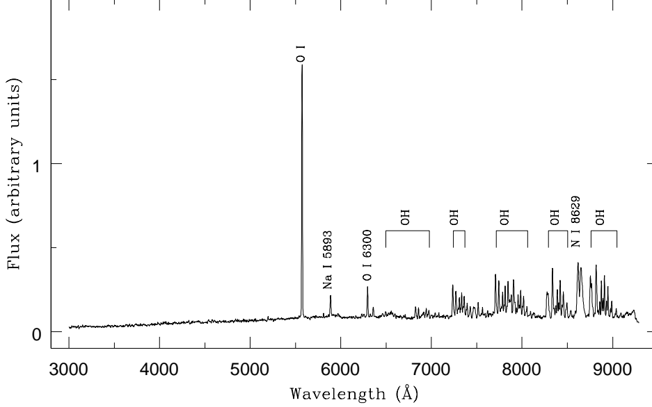
Figure 7. Night sky spectrum at IAO, Hanle. Prominent sky lines are marked.
