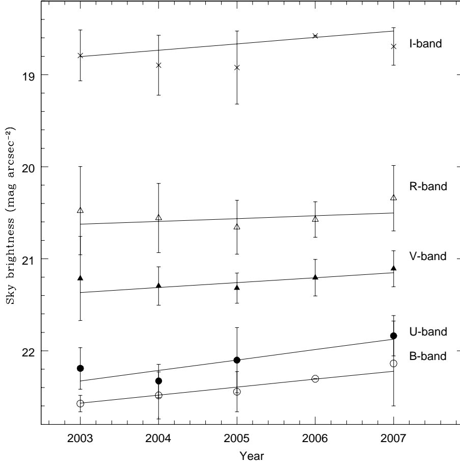
Figure 4. Yearly variation of night sky brightness in UBVRI bands. The solid line is the unweighted linear least squares fit to the data. The error bars represent the scatter in the average values, the accuracy of individual measurements being much smaller. For the B and I bands in 2006 only one measurement is available in each band and hence the error bars are not plotted.
