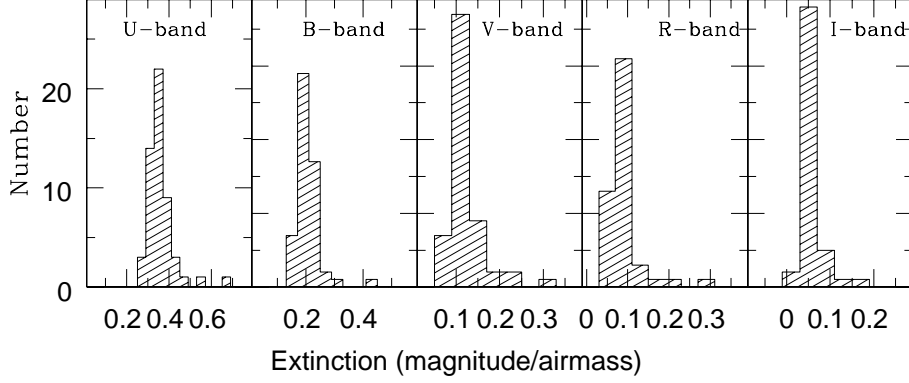
Figure 1. Distribution of the measured extinction coefficients in magnitude/airmass at IAO in UBVRI bands
