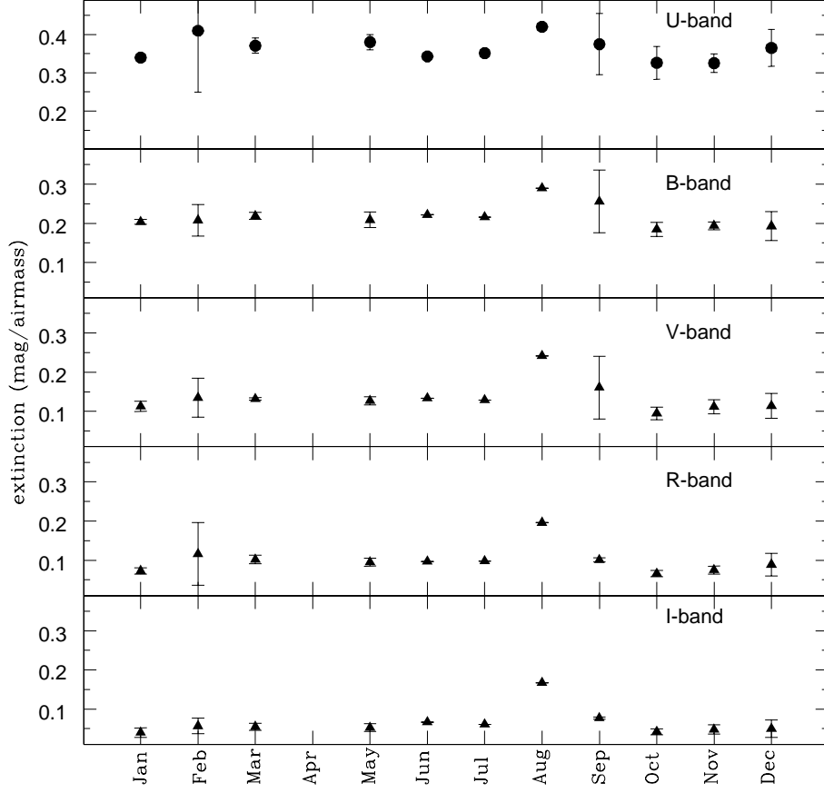
Figure 2. Monthly variation of extinction at IAO during the period 2003–2007. The error bars when not visible are less than the size of symbols. These error bars represent the scatter in the values, the accuracy of individual measurements being much smaller.
