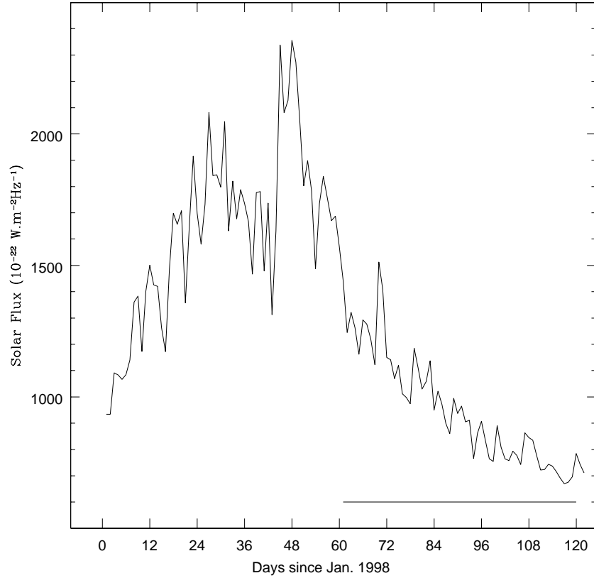
Figure 5. Average monthly solar flux at 10.7 cm since January 1998. The horizontal bar indicates the period (2003–2007) of sky brightness results presented here.
