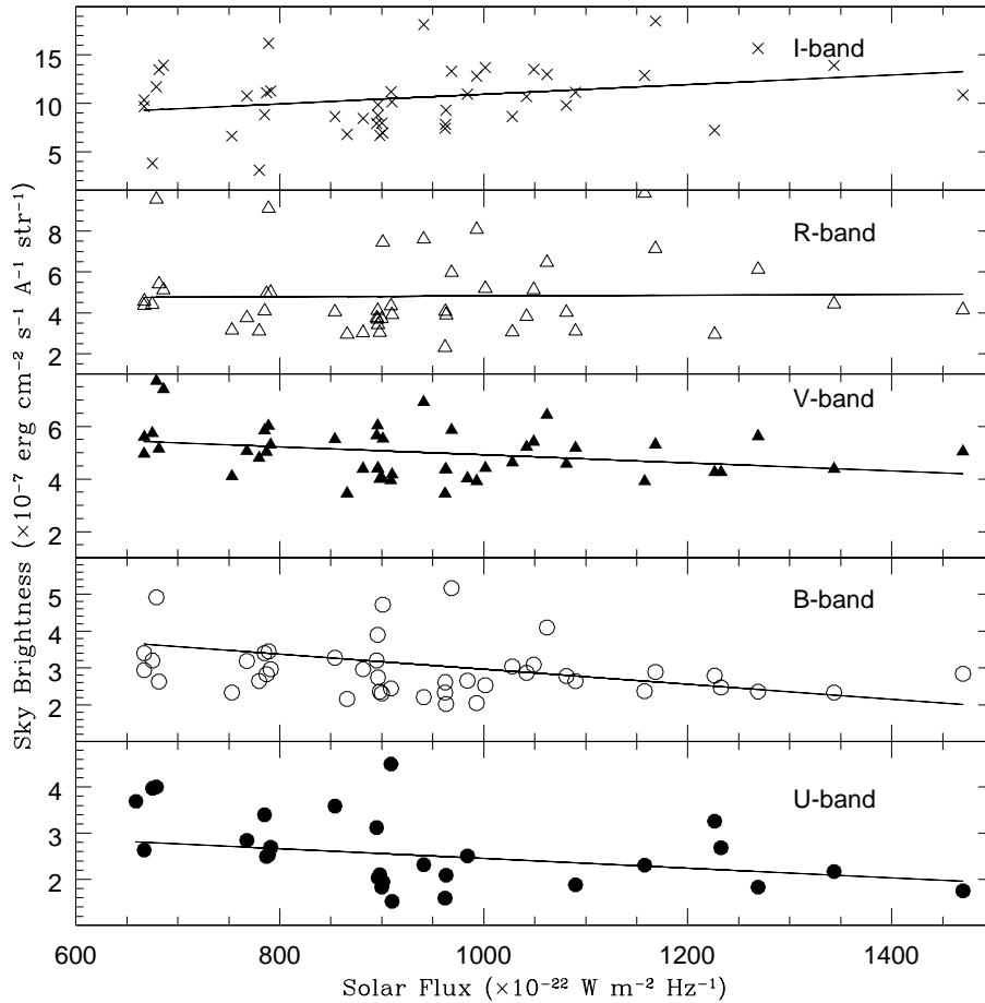
Figure 6. Variation of sky brightness with solar flux density at 10.7 cm. The solar flux density values are 10 days average prior to the date of measurement of sky brightness. The solid line is the linear least squares fit to the data.
