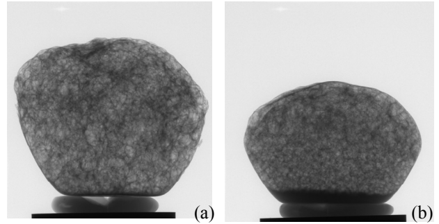
Figure 2. X-ray images of \text{Al-TiB}_2 composite foam after 200 s of holding (a) without Al dilution (6 vol.% of \text{TiB}_2 particles = #3) and (b) with Al dilution to 2 vol.% \text{TiB}_2 (#4), both foamed with untreated \text{TiH}_2 . Bottom part of the foam is 30 mm wide.
