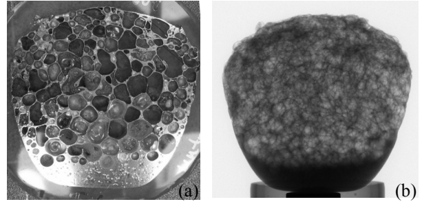
Figure 1. (a) Cross section and, (b) X-ray image of \text{TiC} stabilized foam (#5). Bottom part of the foam is 30 mm wide.
