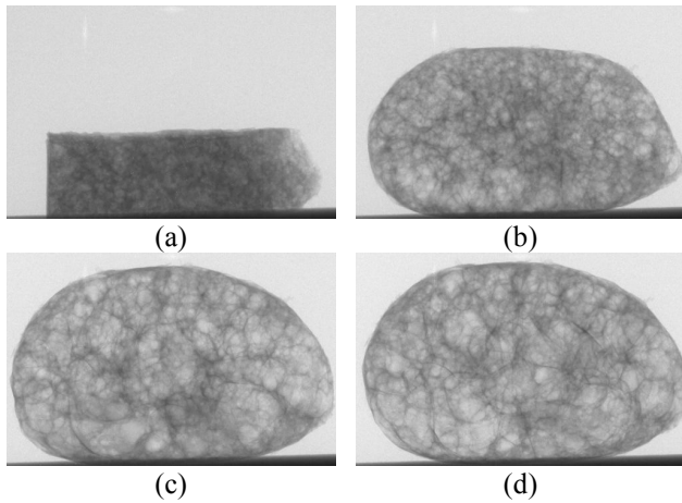
Figure 5. \text{TiB}_2 stabilized foam evolution: (a) precursor in solid state, (b) foamed and melted precursor at 700^\circ\text{C} after 100 s, (c) after 200 s and (d) after 600 s holding.
