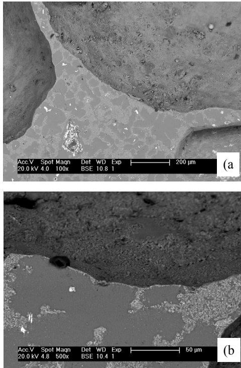
Figure 3. SEM images of Al-TiB 2 foam showing (a) cell walls and a Plateau border with TiB 2 particles in interdendritic regions, (b) TiB 2 layer segregated on cell surface.
