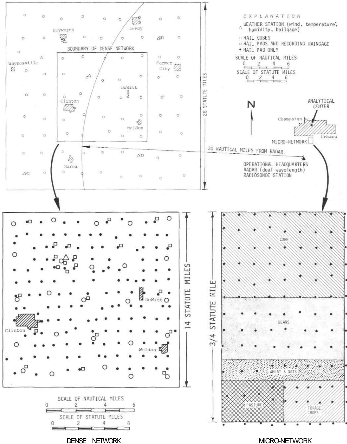
Figure 7. The Illinois State Water Survey surface hail observing networks
