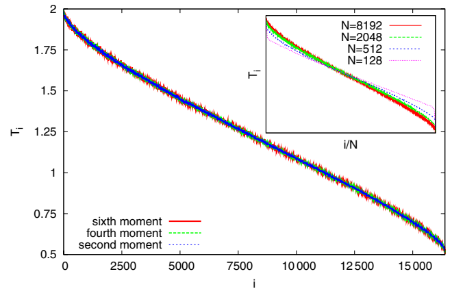
FIG. 2 (color online). Kinetic temperature profile for a FPU- \beta chain with N = 16384 , T_L = 2.0 , T_R = 0.5 , and \gamma = 2.0 . The first three even moments of the velocity are shown; their agreement indicates a Gaussian velocity distribution. (Inset) Normalized temperature profiles for different N .
