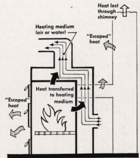
Heating plant efficiency
