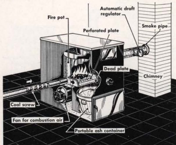
Anthracite cross-feed burner
