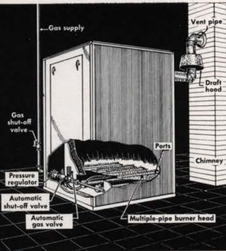
Gas burner with multiple-pipe burner head
