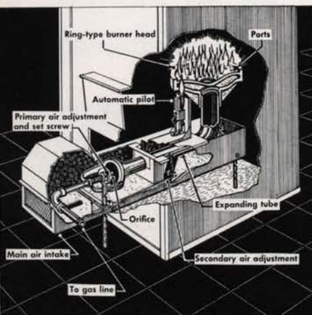
Detail of ring-type gas burner
