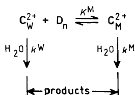
Scheme 1. C^{2+} = cis-[Co(en)_2(C_6H_{11}NH_2)Cl]^{2+} .
