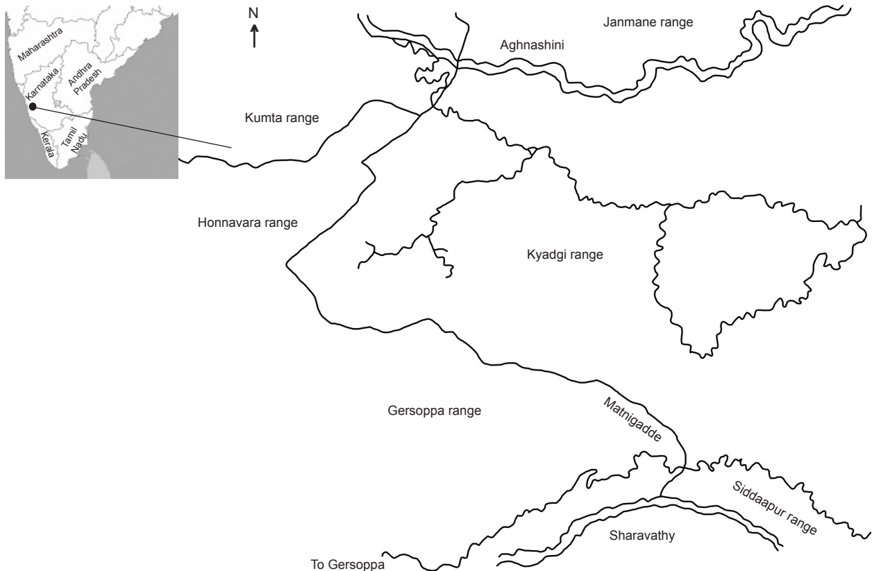
Figure 1. Map of the study area. Aghnashini and Sharavathy are the major rivers and other place names indicate forest ranges
