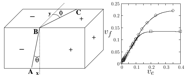
FIG. 1: (left) The geometry of our simulation cell. Ising spins are defined over a 14 \times 14 \times 30 lattice elongated in the z direction. An external field is imposed which changes sign over a plane A, B, C making angles \theta and \phi with the x and y axes respectively. The plane A, B, C moves to the right with velocity v_e . (right) A plot of the velocity of the Ising interface v_f as a function of v_e for two different orientations - (0, 2/7) (top) and (2/7, 2/7) . Note that for small v_e , the interface follows the field ( v_f = v_e ) but gets detached at higher velocities.
