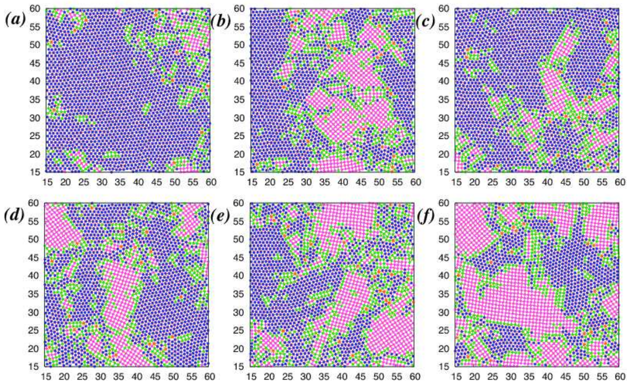
FIG. 13: [Color Online:] Evolution of configurations showing square-triangle coexistence with increasing force (a) F = 90 , (b) 95, (c) 100, (d) 105, (e) 110, and (f) 115, together with the computed Delaunay mesh. The particles are colored according to the number of neighbors n = 4 (magenta), 5 (green), 6 (blue) and 7 (orange). Particles with coordination 5 are present mainly in the interfacial region while those with 7 are associated with isolated dislocations.
