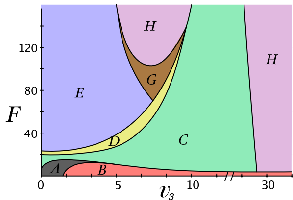
FIG. 1: [Color Online]: Schematic Dynamical Phase Diagram of our model system, plotted as a function of the three-body interaction strength v_3 and of driving force F (see text for a more detailed discussion). The phases are (A) pinned triangular (B) pinned square (C) plastic flow (D) anisotropic hexatic (E) flowing triangular (G) coexistence regime and (H) flowing square. The precise location of the lines separating these phases is disorder-dependent, although the general topology of the phase diagram is not sensitive to disorder. The boundary separating plastic flow from the flowing square phase is a very strong function of the driving force F at large v_3 .
