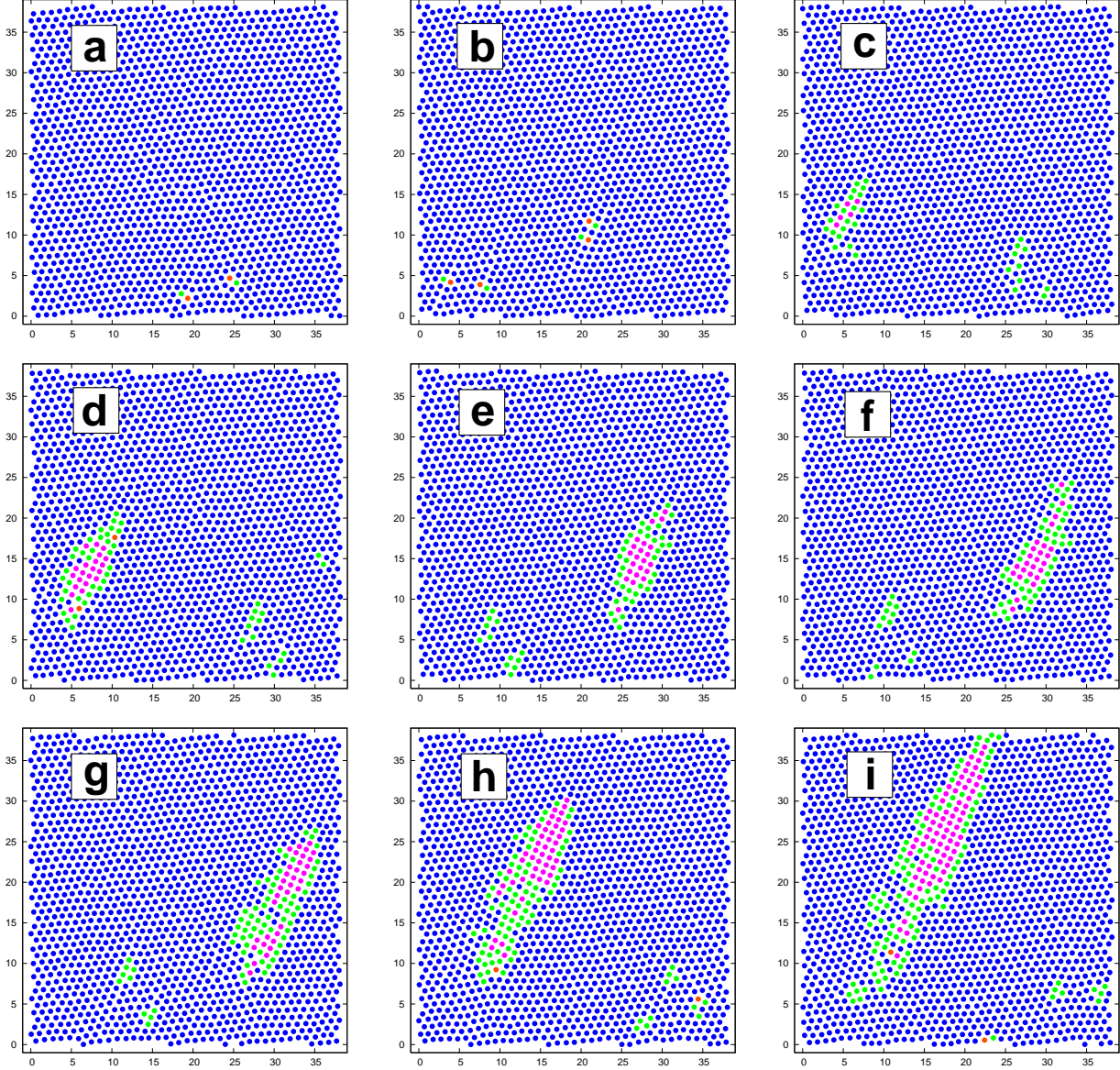
FIG. 15: [Color Online:] Dynamical nucleation of a square defect against a triangular background, shown for F = 98 , v_3 = 6.0 and at TimeSteps = 60 \times 10^3(a) , 70 \times 10^3(b) , 80 \times 10^3(c) , 84 \times 10^3(d) , 86 \times 10^3(e) , 90 \times 10^3(f) , 94 \times 10^3(g) , 96 \times 10^3(h) , 10^5(i)
