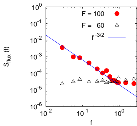
FIG. 17: [Color Online:] The power spectrum S_{flux}(f) of current fluctuations in the moving triangle phase (open triangles F_x = 60 ) and in the coexistence region (red circles F_x = 100 ), logarithmically binned and plotted for a range of frequencies below the washboard frequency. Current fluctuations in the coexistence region are enhanced , also showing a 1/f^{3/2} decay in the low frequency range.
