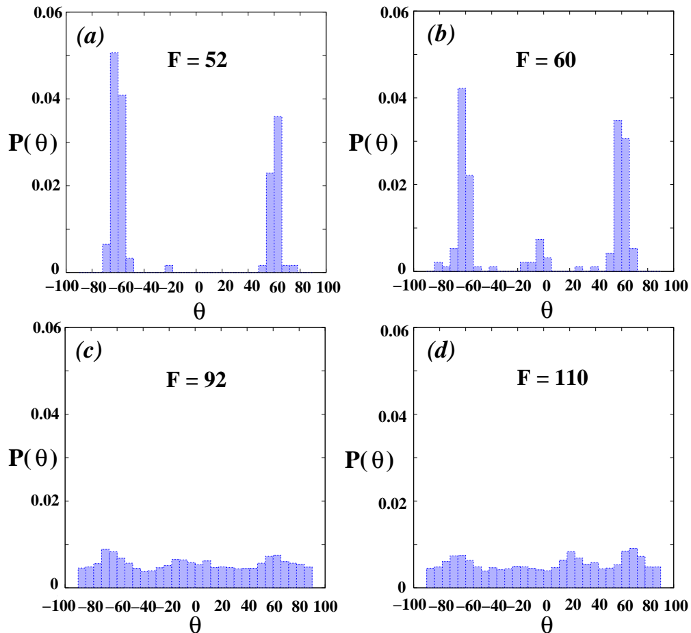
FIG. 16: [Color Online:] The distribution of the angle made by the major principal axis (the eigenvector corresponding to the eigenvalue \lambda_> ) of the square islands within a triangular background, computed for different values of the driving force F . The force values are (a) F = 52 , (b) F = 60 , (c) F = 92 and (d) F = 110 , with v_3 = 6 .
