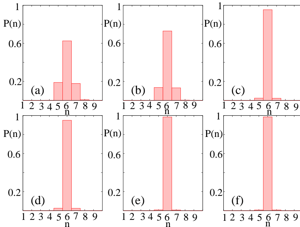
FIG. 3: [Color Online]:The coordination number probability distribution at successive stages of freezing of the driven liquid, at driving forces F_x = 6(a) , 10(b) , 20(c) , 22(d) , 32(e) and 40(f) and with v_3 = 6 . These forces correspond to the forces given in the configuration snapshots of Fig. 2.
