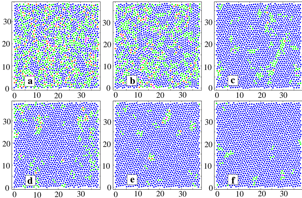
FIG. 2: [Color Online]: Instantaneous snapshots of steady state configurations of the system at T = 0.1 with v_3 = 6.0 . The configurations (a) - (f) are respectively for driving forces F_x = 6, 10, 20, 22, 32 and 40 respectively. The particles are colored according to their coordination number n = 4 (magenta), 5 (green), 6 (blue), 7 (orange) and 8 (grey), as obtained from Delaunay triangulations.
