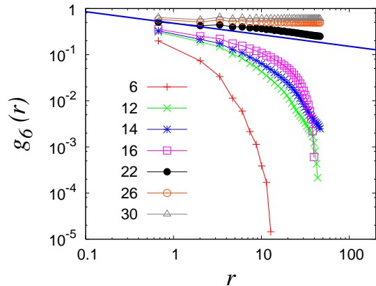
FIG. 5: [color Online]: The hexatic correlation function g_6(r) for F = 6, 12, 14, 16, 22, 26 and 30 , each averaged over 50 independent configurations of a N = 10000 particle system at v_3 = 6 . The solid line indicates the universal behavior g_6(r) \sim r^{-1/4} at the liquid to hexatic transition.
