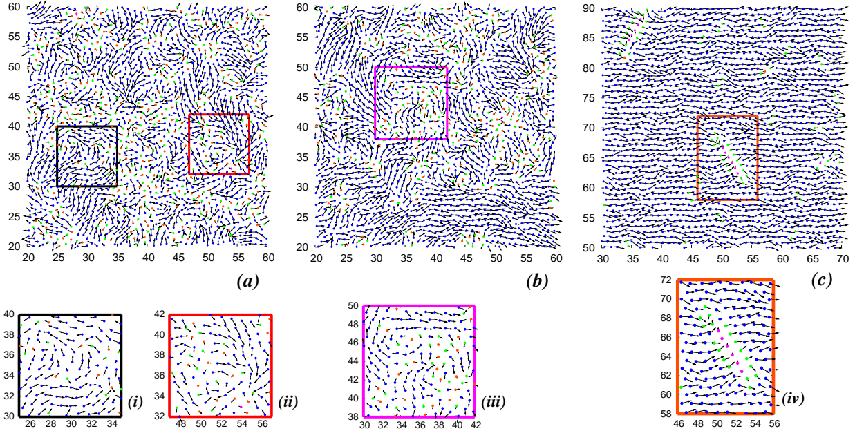
FIG. 8: [Color Online]: Typical orientation of the ‘hexatic-spins’ (see text) associated with particles in the liquid (a), anisotropic-hexatic (b) and triangular (c) phases, at the driving forces F_x = 10, 24 and 40 respectively. The boxes in (a), (b) and (c) are expanded in (i) and (ii) (corresponding to the configurations boxed in (a)), in (iii) (corresponding to the configuration boxed in (b)) and (iv), corresponding to the boxed configuration in (c), to enable an easier visualization of spin configurations. The colors correspond to local coordination, n = 6 (blue), 5 (green), 4 (magenta) and 7 (orange). Note the presence of extended defects in the ordering shown in (c), associated with “strings” with local square symmetry. In all the three pictures only a part of the simulation box is shown for the sake of clarity and the configurations are obtained for v_3 = 6 .
