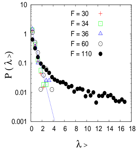
FIG. 9: [Color Online]: Probability distribution of the largest eigenvalue \lambda_> in a semi-logarithmic scale for external forces F = 30, 34, 36, 60 and 110 . It is clear that for all but the largest force, the probability distribution is exponential showing that the energy of string-like excitations within the triangular phase is linear with size. For the largest force which is inside the coexistence region (see text), the probability distribution decays slower than an exponential.
