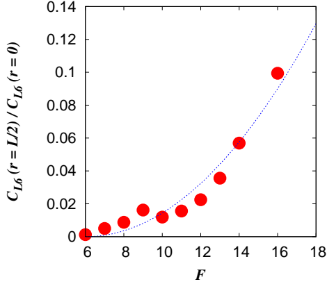
FIG. 12: [Color Online:] The constant part in the angular correlation function along the drive direction goes quadratically with the driving field strength above F_c as predicted by Fertig et al. [67]. The data points (circles) are for v_3 = 6.0 and the dashed line is a guide to the eye.
