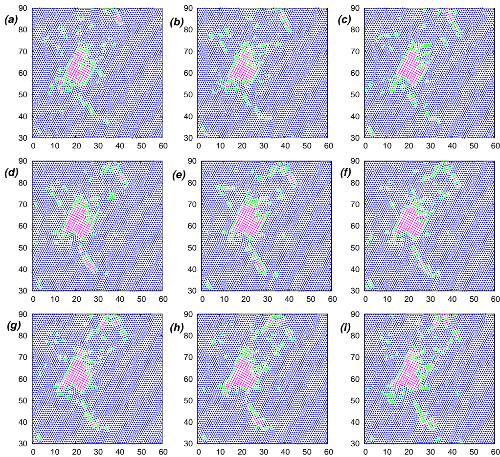
FIG. 19: [Color Online:] Configuration snapshots arising from a quench to zero force of a randomly chosen configuration within the coexistence regime, at time steps (a) 0, (b) 4 \times 10^3 , (c) 10^4 , (d) 5 \times 10^4 , (e) 10^5 , (f) 2 \times 10^5 , (g) 3 \times 10^5 , (h) 5 \times 10^5 , and (i) 9 \times 10^5 , with v_3 = 6.0 . The system size is N = 10000 .
