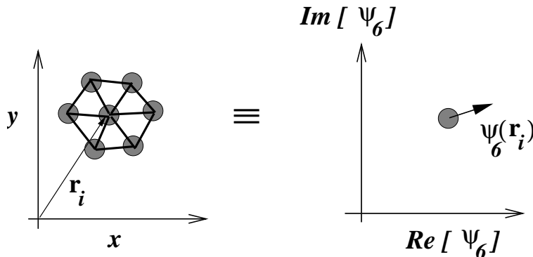
FIG. 7: Mapping to the XY model : local hexagonal configuration around the particle i (diagram on left) may be analyzed in terms of the phasor \psi_6(\mathbf{r}_i) represented as a spin situated at \mathbf{r}_i (diagram on right).
