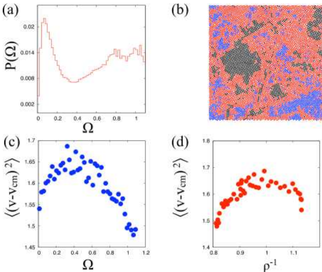
FIG. 18: [Color Online:] (a) Probability distribution of the bond angle order parameter \Omega (see text) in the coexistence regime. The peak at low value of \Omega corresponds to the square phase. The series of peaks at high \Omega values all correspond to various combinations of bond angles in the (disordered) triangular phase. The interfacial region has \Omega corresponding to the first dip in the curve. (b) Illustration of the spatial distribution of \Omega values as stated in (a) \Omega < 0.2 (square) are black, those for 1.3 > \Omega > 0.2 are red (interface) and those for \Omega > 1.3 are blue (triangle). (c) The fluctuation of the local velocity about the centre of mass value \langle (v - v_{cm})^2 \rangle plotted against \Omega . It is clear that the fluctuations are largest for the particles in the interfacial region. (d) The fluctuation of the local velocity as a function of the local volume per particle.
