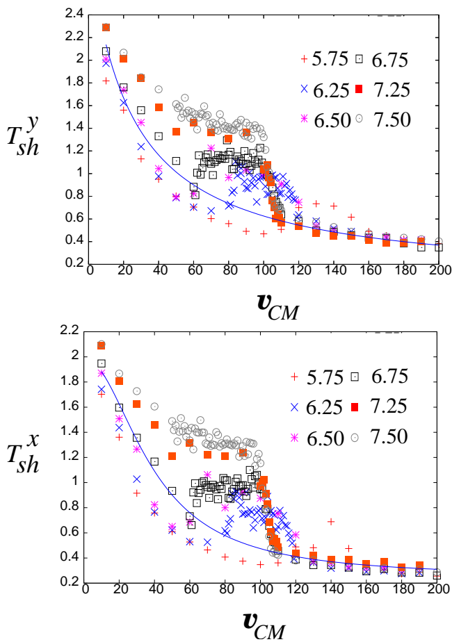
FIG. 14: [Color Online]: The shaking temperatures in the transverse (top) and drive (bottom) directions ( T_{sh}^y and T_{sh}^x ) for different v_3 as a function of the centre of mass velocity ( v_{CM} ), showing the quantity is almost independent of v_3 except in and around the coexistence regime, due to effects of fluctuation.
