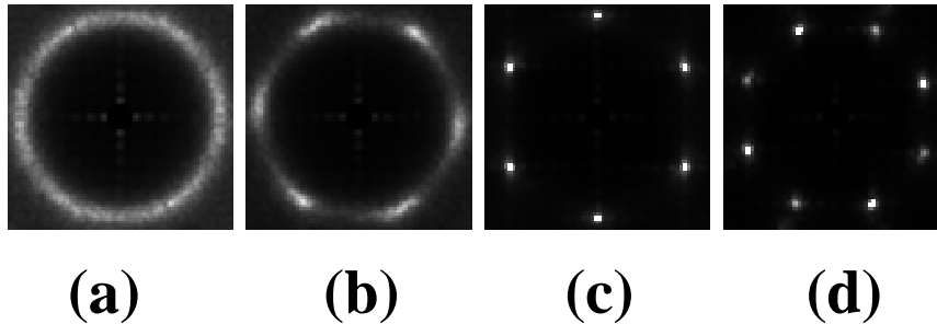
FIG. 4: Structure factor S(\mathbf{q}) for the plastic flow state (a), anisotropic hexatic phase(b), moving triangle (c) and moving square solid phases (d) at v_3 = 6.0 and F_x = 10, 20, 60 and 140 respectively. To obtain S(\mathbf{q}) , 50 independent configurations were used. The structure in (d) reflects the presence of two misoriented square crystallites.
