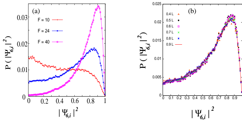
FIG. 6: [Color Online:] (a) The distribution of the amplitude of the local hexatic order parameter |\psi_{6,i}|^2 over the system for N = 10000 in the plastic ( F_x = 10 ), hexatic-glass ( F_x = 24 ) and moving triangular ( F_x = 40 ) regimes, with v_3 = 6.0 (b) Scaling of the distribution of |\psi_{6,i}|^2 deep in the hexatic regime for F_x = 26 , computed over fractions 0.4, 0.5, 0.6, 0.7, 0.8 and 0.9 of the simulation box length L , with v_3 = 6.0 .
