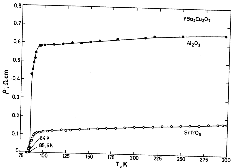
Figure 1. Resistivity vs temperature curves for \text{YBa}_2\text{Cu}_3\text{O}_7 screen printed films on \text{Al}_2\text{O}_3 and \text{SrTiO}_3 substrates ( 950^\circ\text{C} , 6 h, air; 600^\circ\text{C} , 6 h, \text{O}_2 ).
