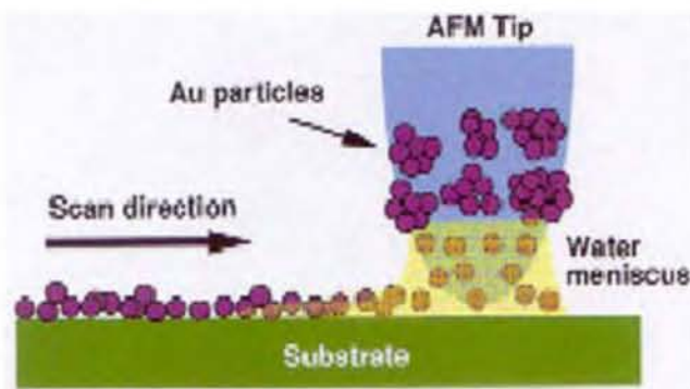
Figure 12. Schematic illustration of the dip-pen process. Au nanocrystals deposited on the cantilever dissolve in the water meniscus between the tip and the substrate. The dissolved nanocrystals are transferred to the substrate, when the tip is slowly scanned across the surface. Aggregates of nanocrystals are formed on the substrate upon evaporation of the water layer.
