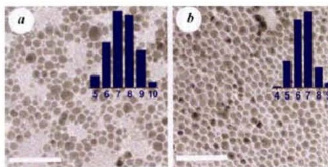
Figure 2. a , TEM image of the as-prepared Au nanocrystals obtained after 24 h from a liquid–liquid interface containing a 1.5 mM solution of Au(PPh 3 )Cl in toluene and 330 \mu l of 50 mM THPC in 16 ml of 6.25 mM aqueous NaOH solution in a 50 ml beaker (bar = 50 nm). b , TEM image of Au nanocrystals obtained starting with a 6 mM toluene solution of Au(PPh 3 )Cl and 1.65 ml of 50 mM THPC in 16 ml of 31.25 mM aqueous NaOH solution (bar = 50 nm). (Inset) Particle size distribution (in nm).
