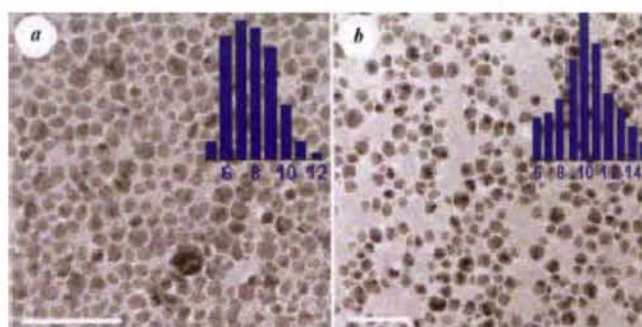
Figure 4. a , TEM image of Au particles obtained at room temperature by reacting a THPC solution in a 3 : 1 water–glycerol mixture and Au(PPh 3 )Cl in toluene layer (bar = 50 nm). b , TEM image of Au particles obtained at room temperature by reacting a THPC solution in a 1 : 1 water–glycerol mixture and Au(PPh 3 )Cl in toluene layer (bar = 50 nm). (Inset) Particle size distributions.
