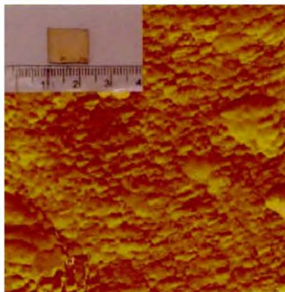
Figure 5. Tapping mode atomic force microscopic image (in phase contrast mode) of an Au film transferred to a highly oriented pyrolytic graphite substrate. The film was prepared starting with 10 mM solution of Au(PPh 3 )Cl in toluene. (Inset) Similar film on a glass substrate.
