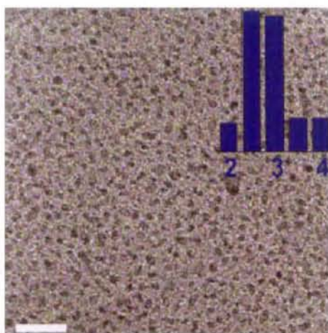
Figure 7. TEM image of Pd nanocrystals obtained at room temperature by reacting a 2.2 mM toluene dispersion of palladium acetate with 330 \mu\text{l} of 50 mM THPC in 16 ml of 6.25 mM aqueous NaOH solution in a 50 ml beaker (bar = 20 nm). (Inset) Particle size distribution.
