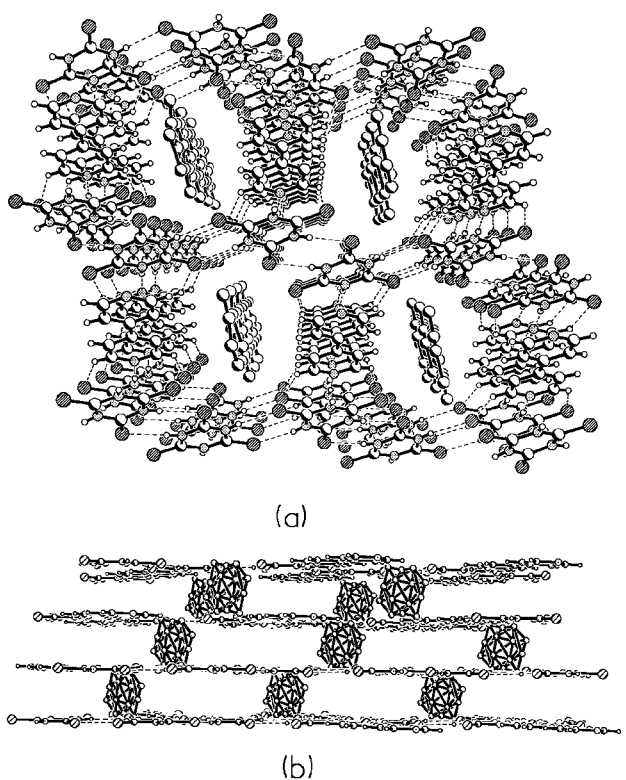
Fig. 2 (a) Three-dimensional structure of the 2:1 TCA-BP co-crystal containing toluene, 2 , in the channels. (b) Stacking arrangement of molecular sheets perpendicular to the channels.
