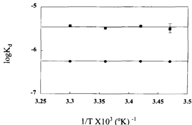
Fig. 7. Van't Hoff plot of tRNA Gln (filled circles) and tRNA Glu (filled squares) binding to glutaminyl-tRNA synthetase, in the presence of ATP. The dissociation constants at four different temperatures, 15, 20, 25, and 30 ^{\circ} C, were determined from tryptophan fluorescence quenching data. The protein concentration was 0.2 \mu M, and the ATP concentration was 1.5 mM. The experiments were conducted in 0.1 M Tris-HCl buffer, pH 7.5 containing 15 mM MgCl 2 . Excitation and emission wavelengths were 295 and 340 nm, and bandpasses were 1.5 and 10 nm, respectively. The error bar shown was the maximum among all the eight points.
