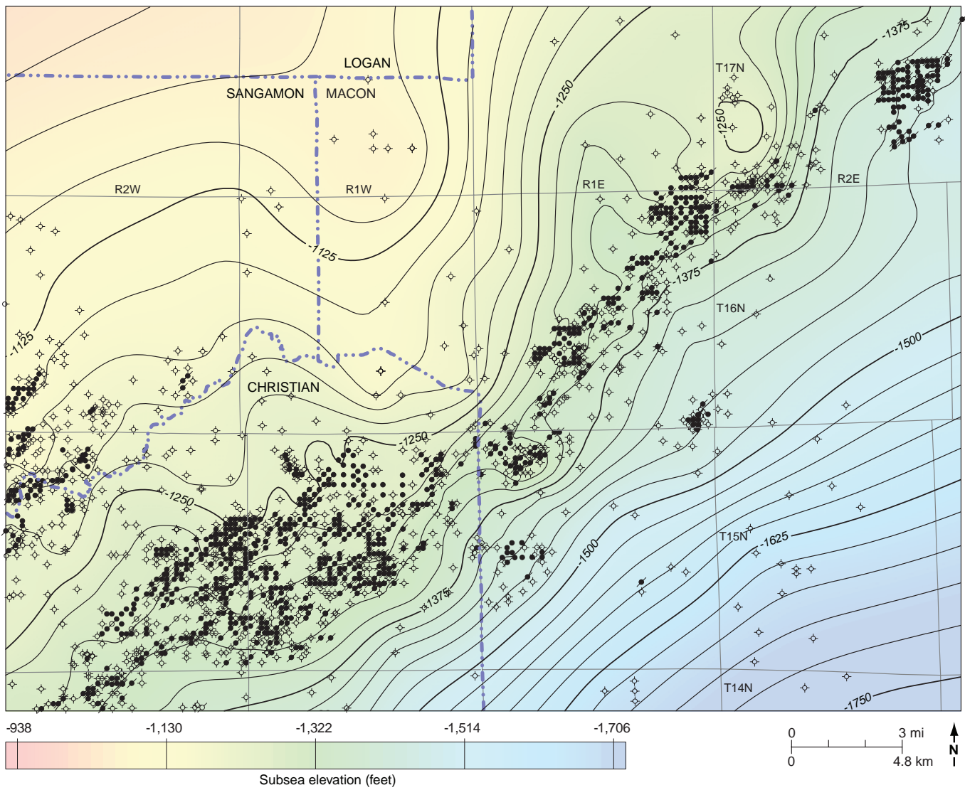
Figure 12 Structure contour map of the base of the New Albany Shale Group showing the direction of the regional dip toward the southeast. Note minor closures and noses that are due to uneven pre-New Albany Shale Group topography.
