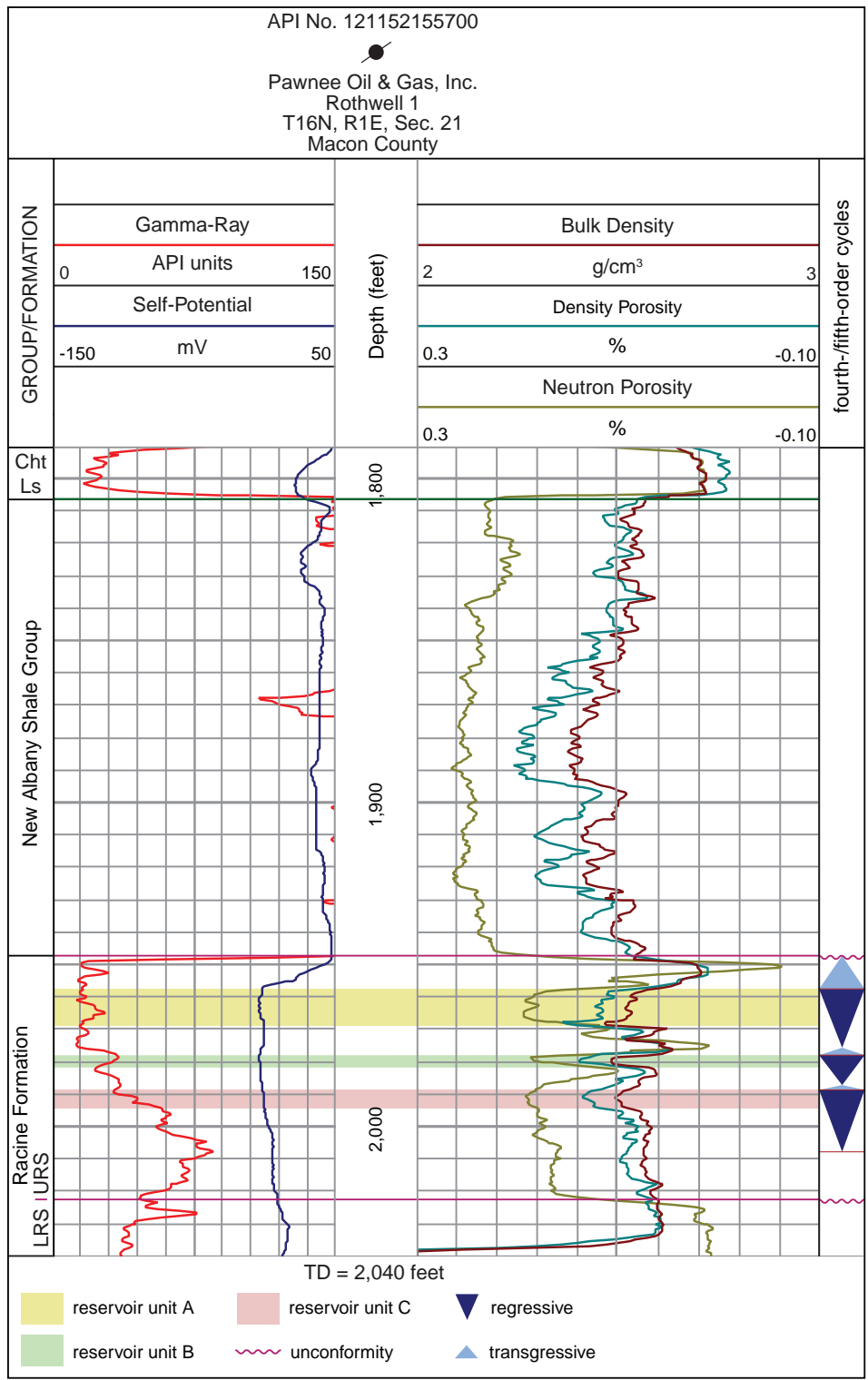
Figure 15 Digitized log of the Pawnee Oil and Gas Inc. Rothwell No. 1 well in the Blackland North Field in Macon County showing the development of non-reef reservoir units A, B, and C in the upper part of the upper Racine sequence. Note the occurrence of the reservoirs in the regressive portion of fourth-order depositional cycles. Abbreviations: Cht Ls, Chouteau Limestone; LRS, lower Racine sequence; TD, total depth; URS, upper Racine sequence.
