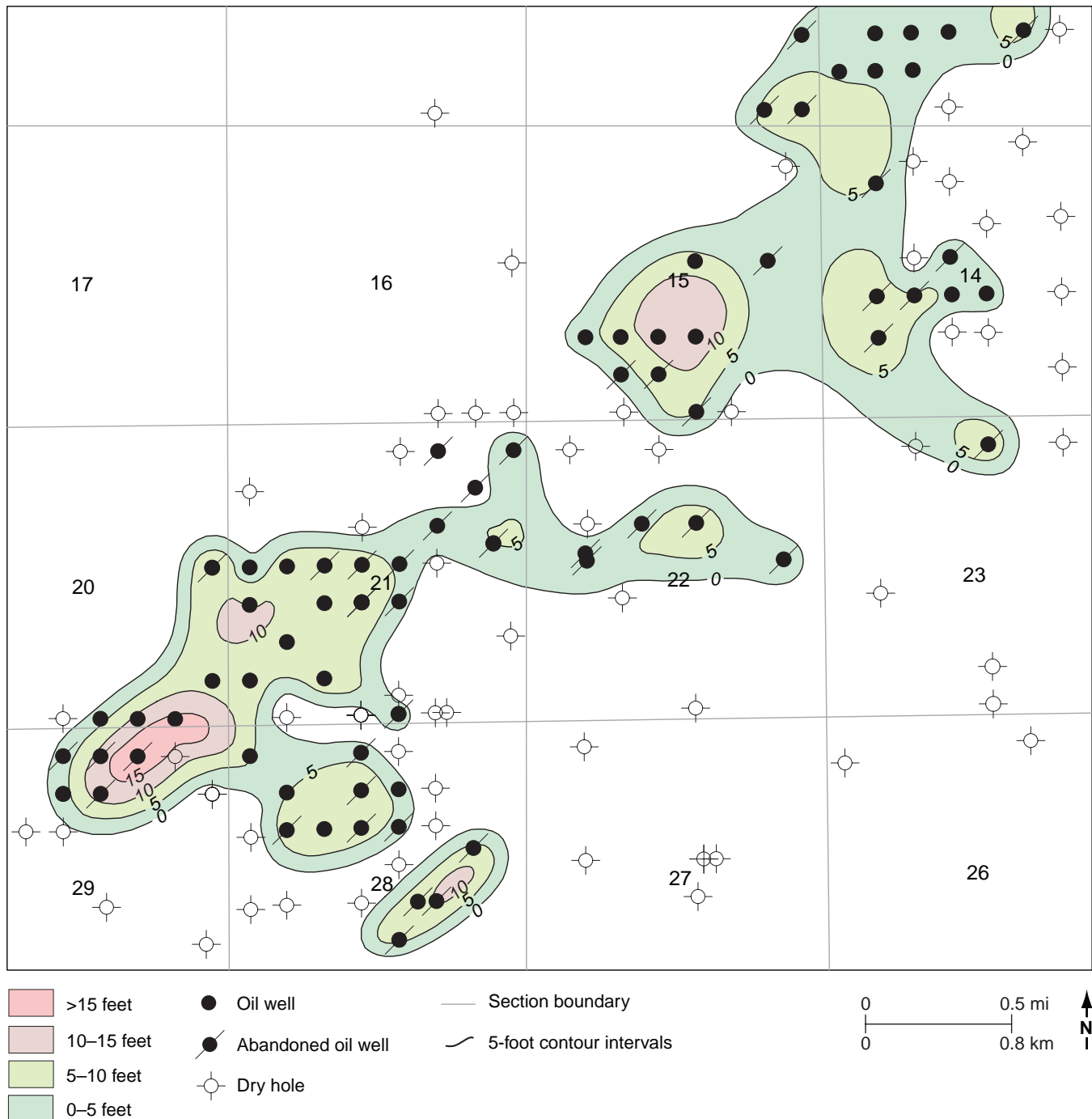
Figure 20 Thickness map showing the lateral distribution of the dolomite reservoir unit C along the Mt. Auburn trend. This lenticular dolomite unit is more extensive than reservoir units A and B and is present in all of the oil fields along the Mt. Auburn trend.
