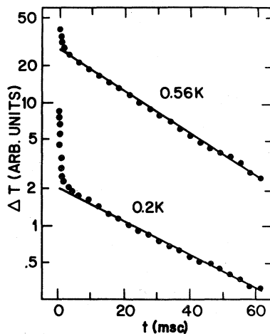
FIG. 3. Exponential behavior of \Delta T(t) at long time scales. The data is taken from the measurements on \alpha\text{-SiO}_2 . The time constant is determined by the heat capacity of the sample and the thermal conductance of the posts. The exponential decay extrapolates to \Delta T_0 = \Delta Q / C_L at zero time, from which the long-time heat capacity C_L can be determined.
