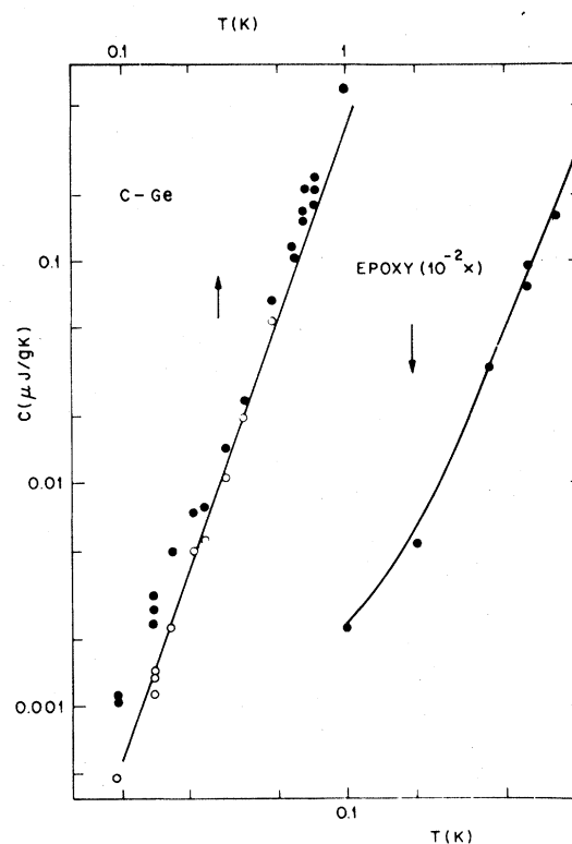
FIG. 9. Left-hand side: the long-time specific heat C_L (solid circles) and the short-time specific heat C_S (open circles) of c\text{-Ge} ; C_D is the Debye heat capacity. The sample weighed 0.645\ \text{g} . Right-hand side: the long-time specific heat C_L of the epoxy Stycast 1266; the sample was 8.7\ \text{mg} .
