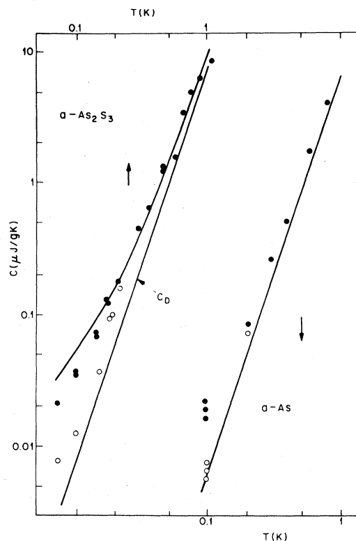
FIG. 8. Long-time specific heat C_L (solid circles) and the short-time specific heat C_S (open circles) of \alpha -As 2 S 3 (left) and \alpha -As (right). The weights of the samples were 0.132 and 0.0838 g, respectively. The thick curves are the specific heats from the measurements of Stephens ( \alpha -As 2 S 3 , Ref. 18) and Jones et al. ( \alpha -As, Ref. 22), and C_D is the Debye specific heat.
