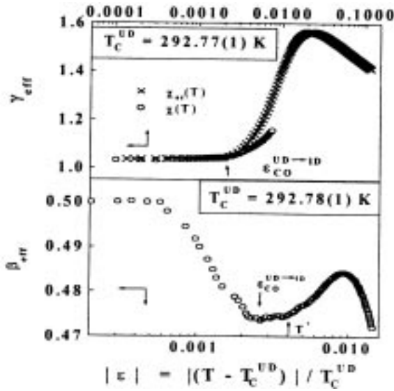
Figure 5. Variation of effective critical exponents, \beta_{\text{eff}} and \gamma_{\text{eff}} , with reduced temperature |\epsilon| (see text).
