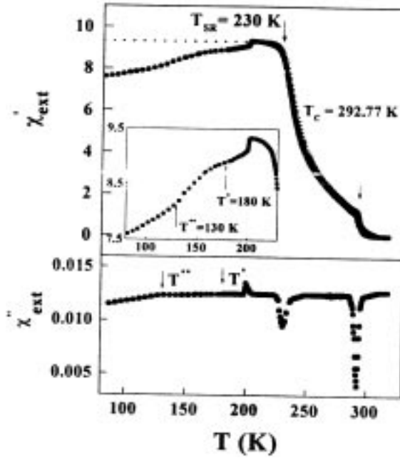
Figure 3. Temperature ( T ) dependence of the real ( \chi'_{\text{ext}} ) and imaginary ( \chi''_{\text{ext}} ) components of ac susceptibility of single crystal sample 1 of Gd at 87 Hz frequency for ac field amplitudes of 10 mOe (closed circles) and 1 Oe (crosses) applied along the c -axis (see text) (ref. [15]). The inset shows expanded plot for the region T = 80 – 230 K. The horizontal dashed line indicates the demagnetisation limited value \chi'_{\text{ext}} = 1/4\pi N_d (see text).
