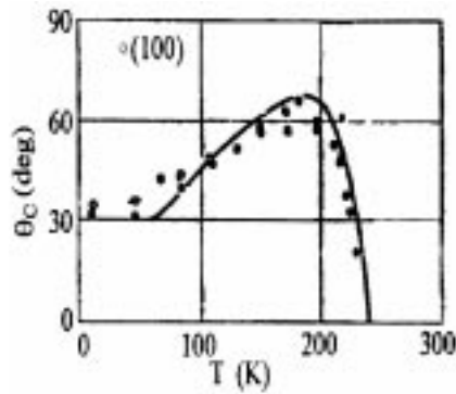
Figure 1. Temperature dependence of the tilt angle ( \theta_C ) of easy direction of magnetisation of Gd with respect to c -axis (ref. [10]).
