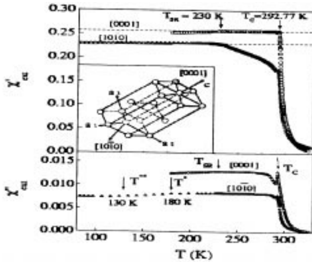
Figure 4. Temperature dependence of the real ( \chi'_{\text{ext}} ) and imaginary ( \chi''_{\text{ext}} ) components of ac susceptibility of single crystal sample 2 of Gd at 87 Hz frequency for ac field amplitude of 10 mOe applied along the crystallographic directions [0001] (open circles) and [10 \bar{1} 0] (open triangles) (ref. [15]). The inset shows the crystal structure of Gd indicating the directions [0001] and [10 \bar{1} 0]. The horizontal dashed lines indicate the demagnetisation limited value \chi'_{\text{ext}} = 1/4\pi N_d (see text).
