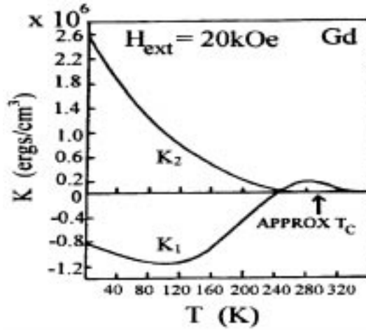
Figure 2. Temperature dependence of magnetocrystalline anisotropy constants K_1 and K_2 of Gd (ref. [9]).
