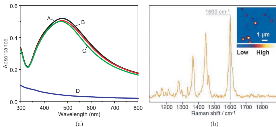
Fig. 6. (a) UV-vis spectrum of Ag@PBT treated with cyanide in water–isopropyl alcohol mixture. The silver core remained stable even for a day in 2 mM NaCN. Curve A indicates the UV–vis spectrum of Ag@PBT in water–isopropyl alcohol mixture. Curve B is the UV–vis spectrum of Ag@PBT measured 1 h after the addition of 2 mM CN − and curve C is after 24 h. Curve D is after adding 10 mM NaCN − . (b) shows the Raman spectrum of Ag@PBT. Inset shows Raman image of the material generated by summing up the intensity at 1600 cm −1 .
